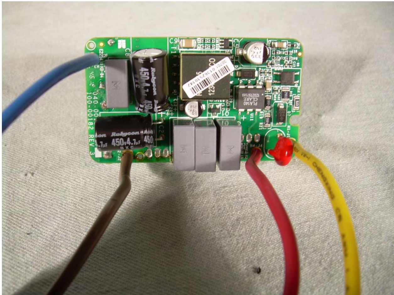
Photograph 15 – Back View of the Main/Power PCB
