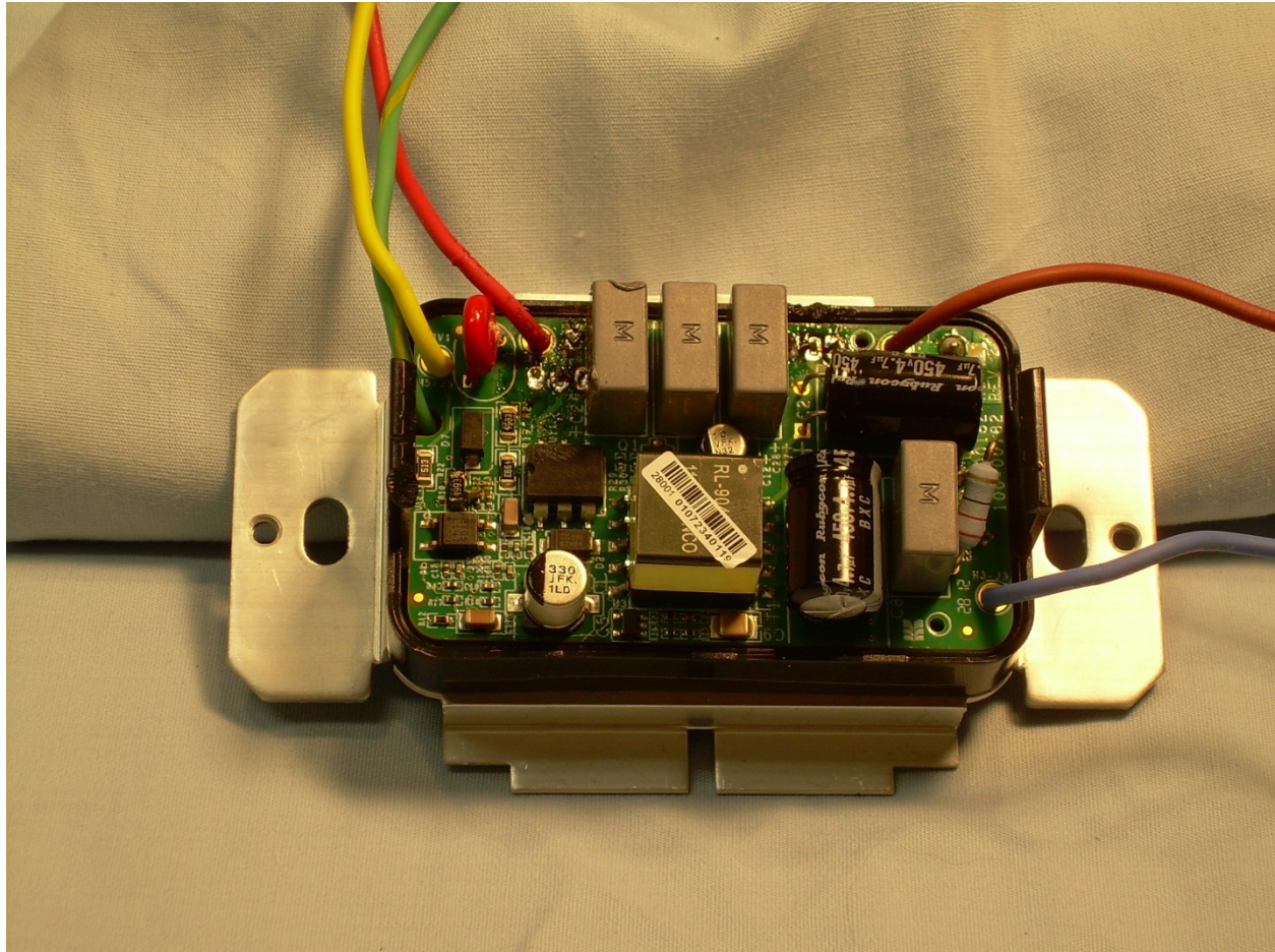
Photograph 13 – View of the EUT with the Back Cover Removed
