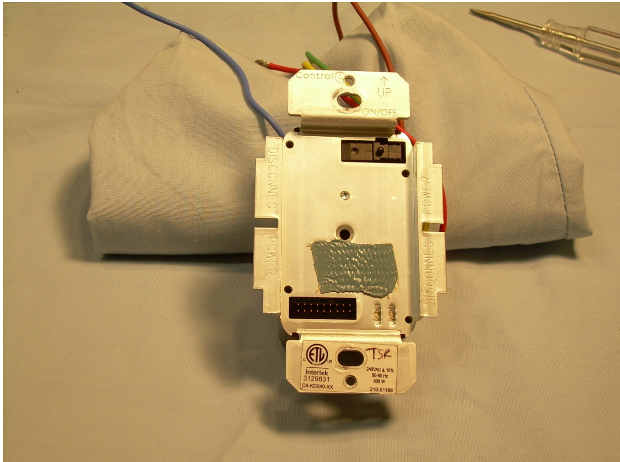
Photograph 12 – View with the RF/Switch PCB and Insulator Removed
