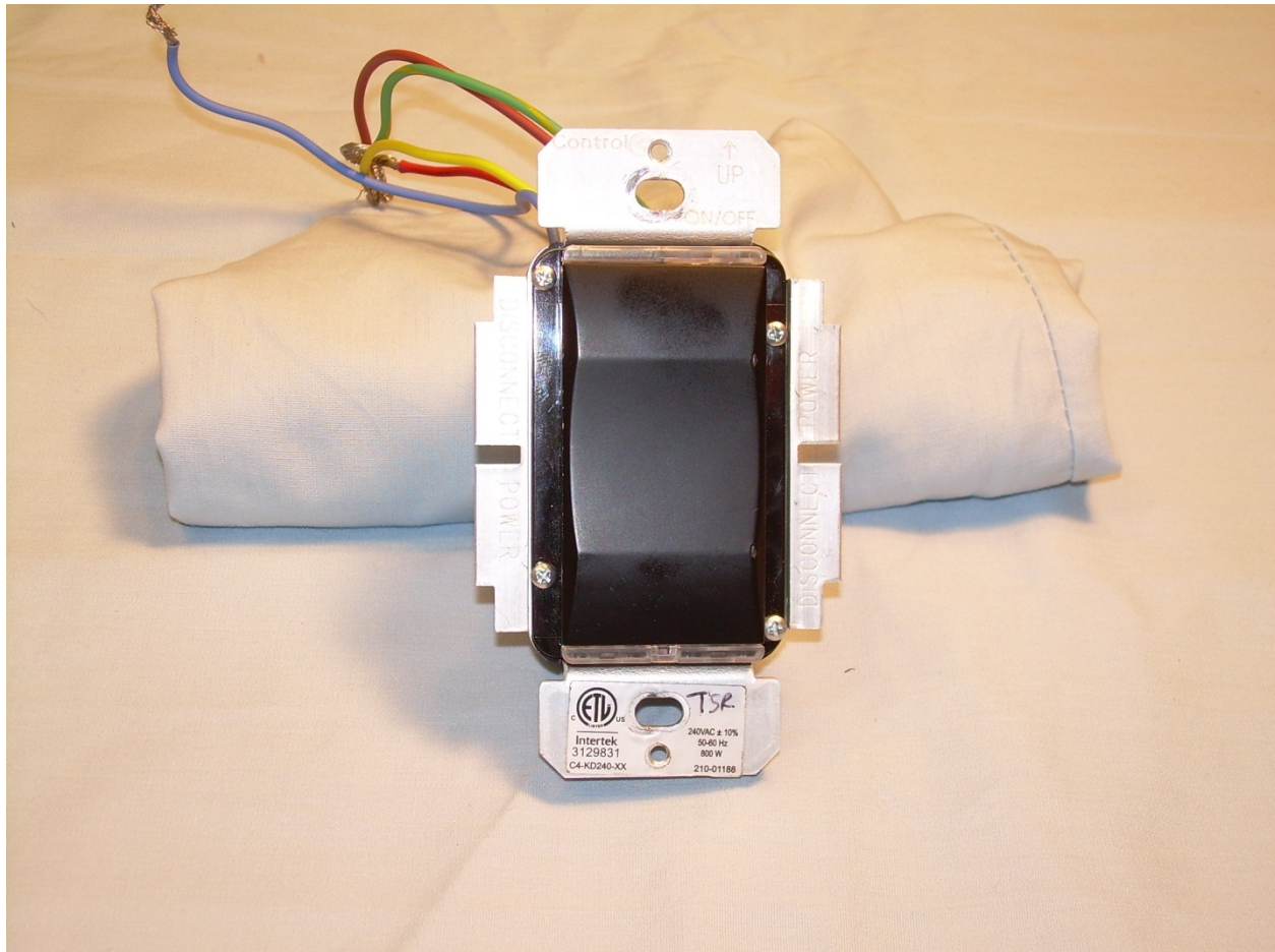
Photograph 5 – Front View of the C4-APD120 and C4-APD277
