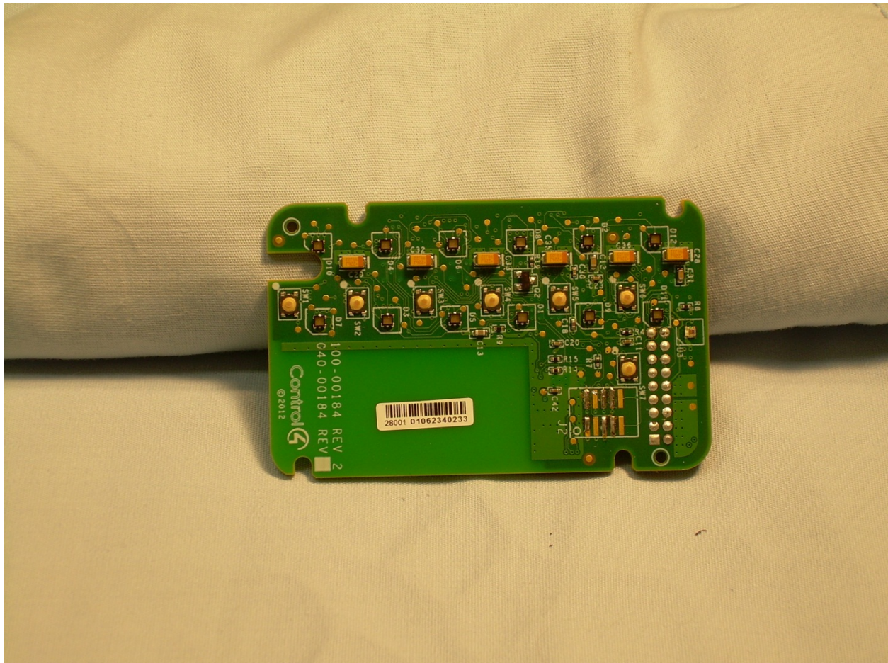
Photograph 9 – Front View of the Switch/RF PCB
