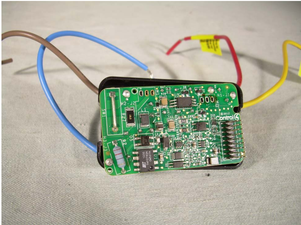
Photograph 14 – Front View of the Main/Power PCB
