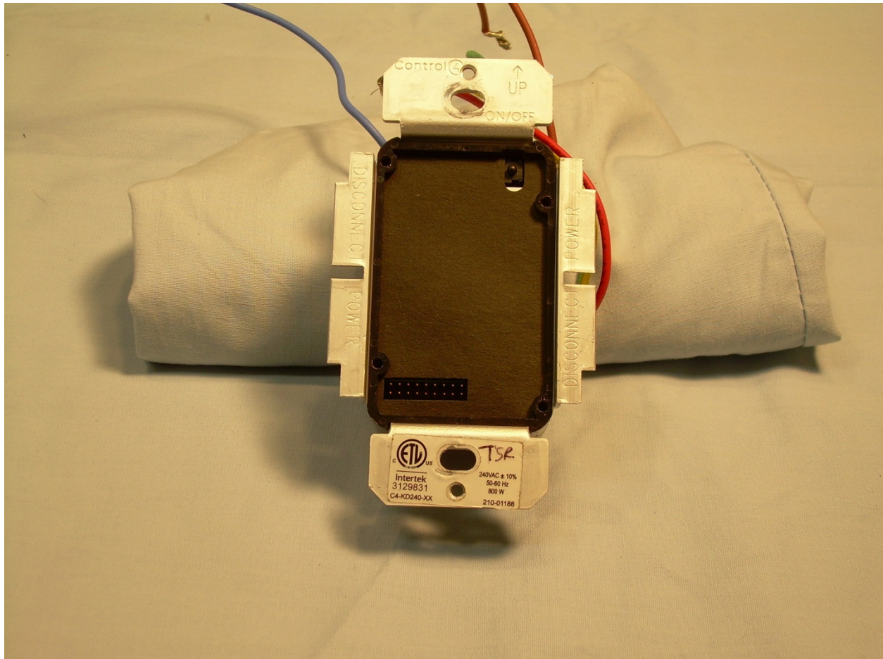
Photograph 11 – View with the RF/Switch PCB Removed
