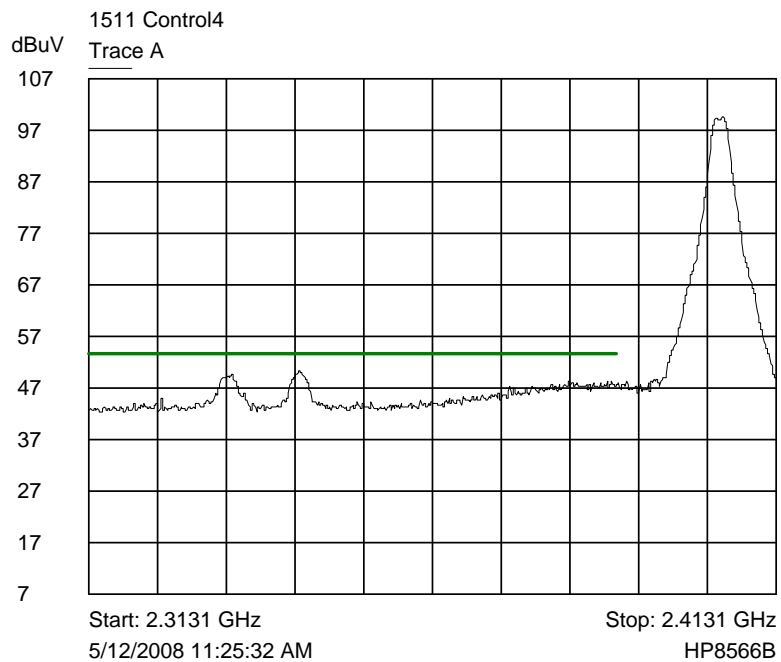
Trace A Lower band edge - radiated - corrected trace
