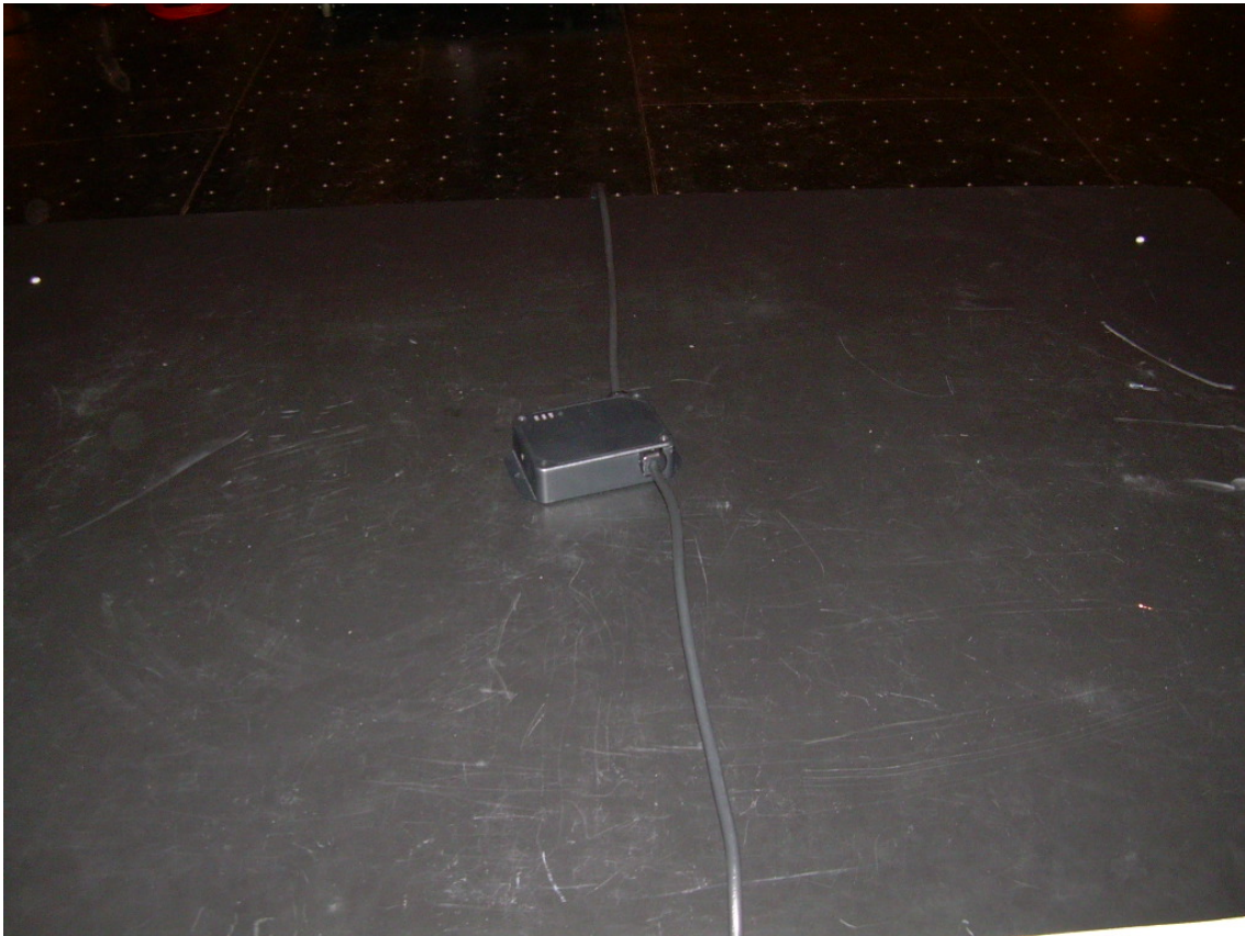
Photograph 1 - View of Radiated Spurious Emissions in the Restricted Bands - Horizontal Setup
