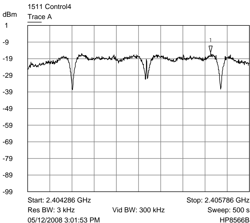
Trace A Lower channel, 3 kHz power spectral density plot
