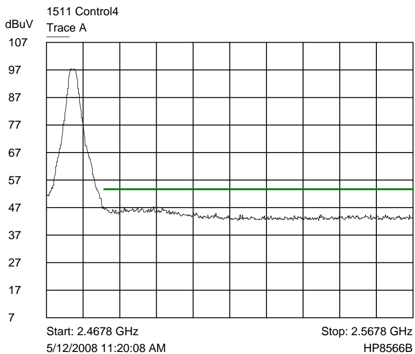
Trace A Upper band edge - radiated - corrected trace
