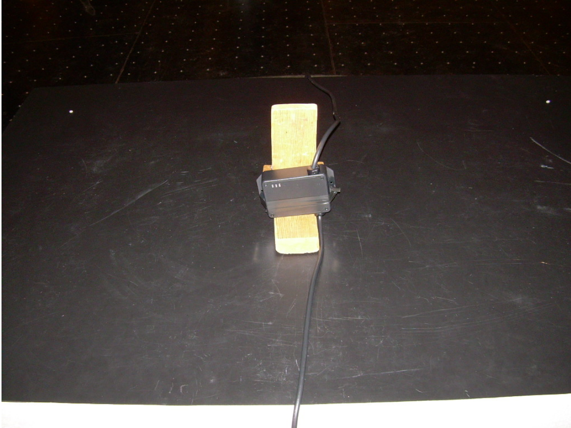
Photograph 3 - View of Radiated Spurious Emissions in the Restricted Bands - On-Edge Setup
