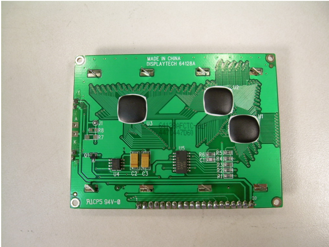
Back View of the Display
