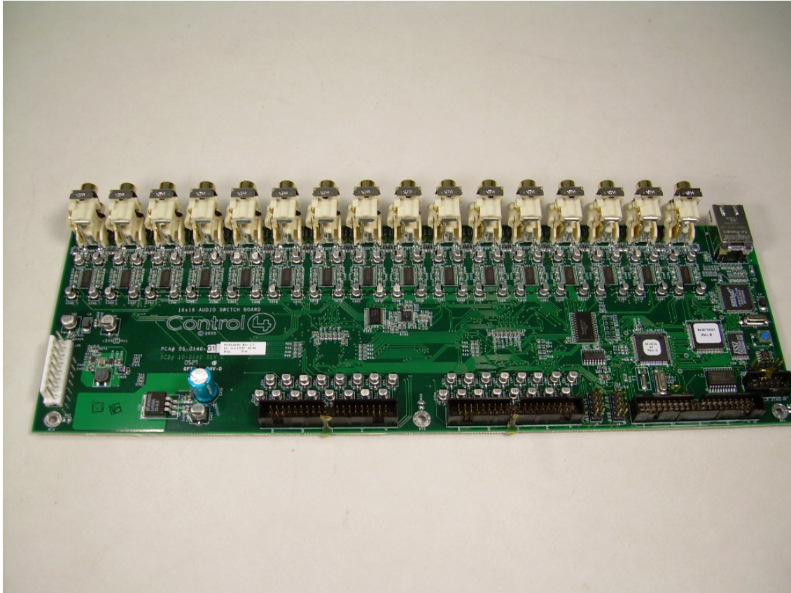
Top View of the Output PCB
