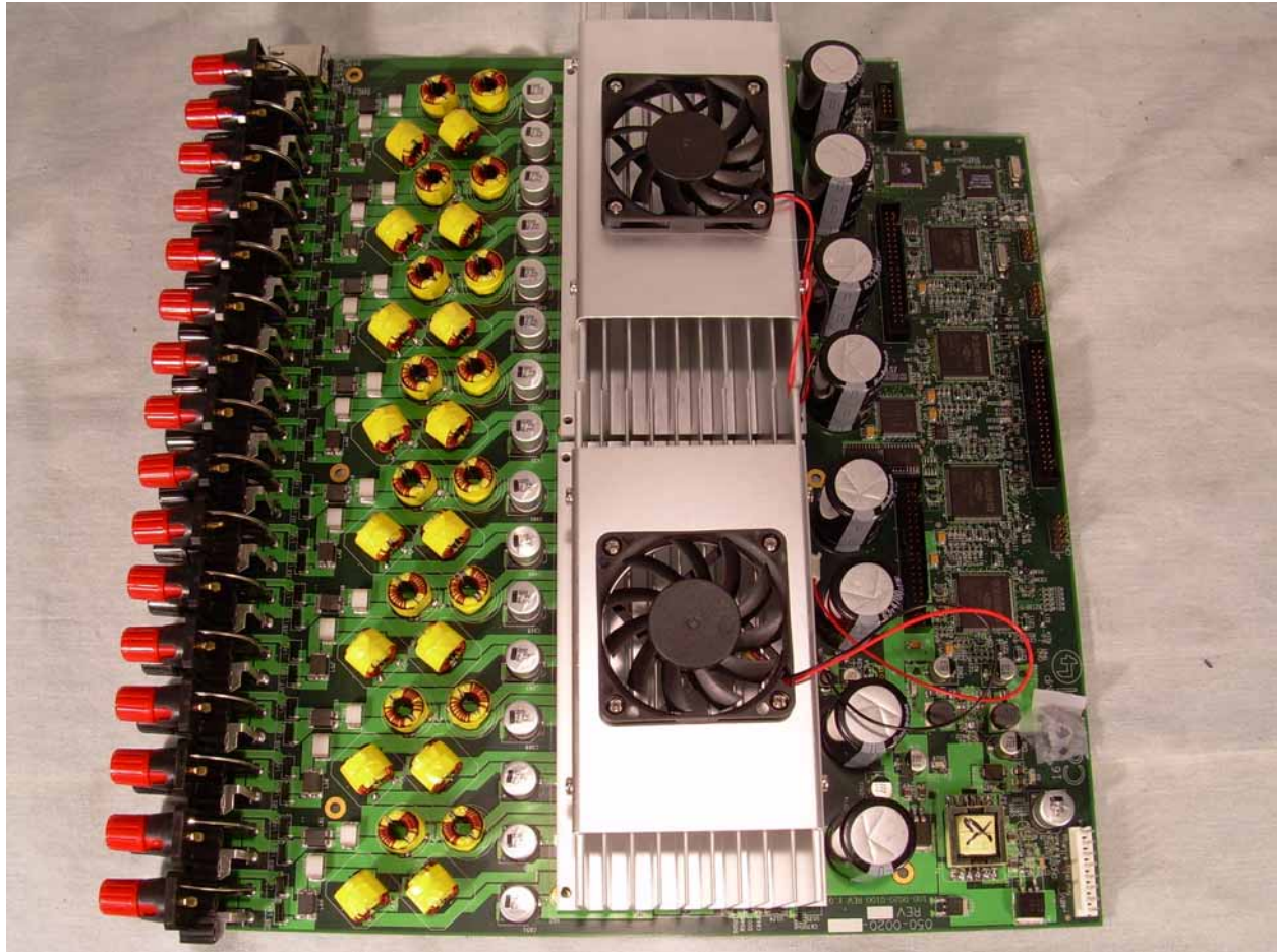
Photograph 8 - Top Side of the Main PCB
