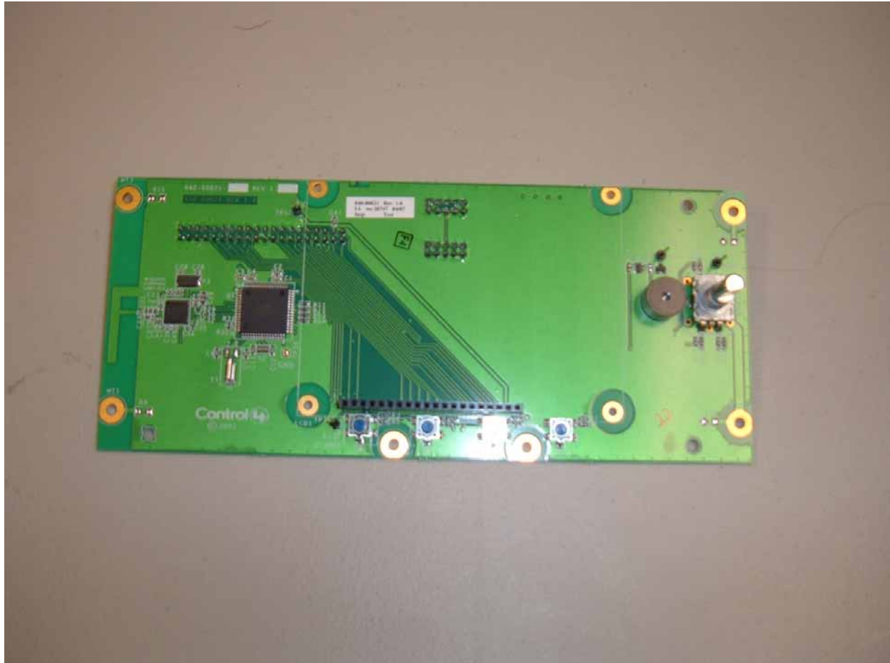
Photograph 14 - Front Side of the Front Panel PCB
