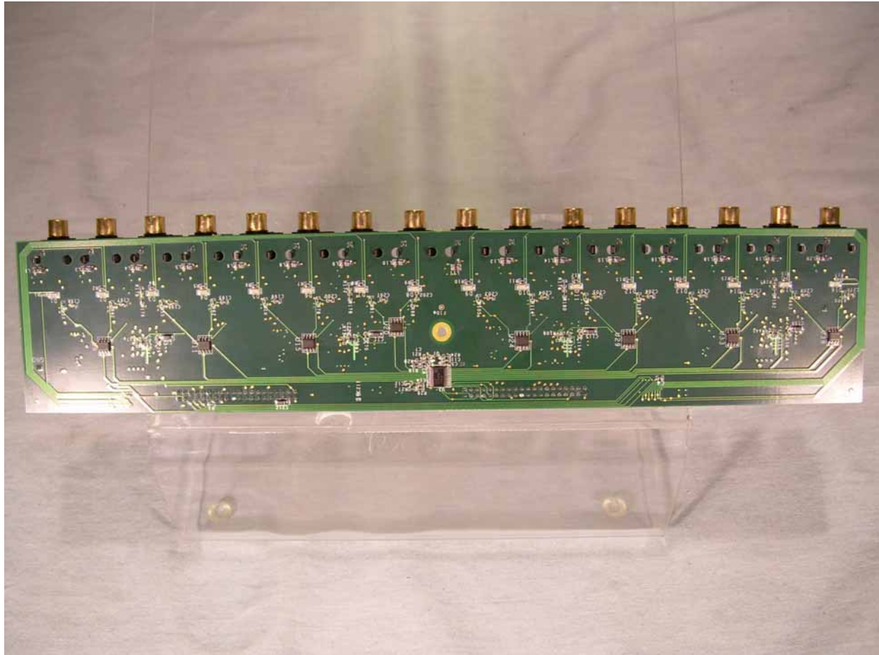
Photograph 11 - Bottom Side of the Rear Panel Interface PCB
