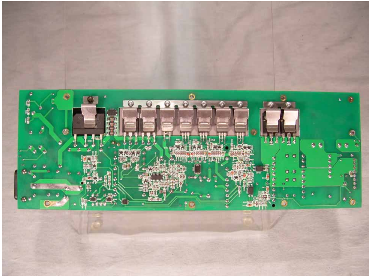
Photograph 13 - Bottom Side of the Power Supply
