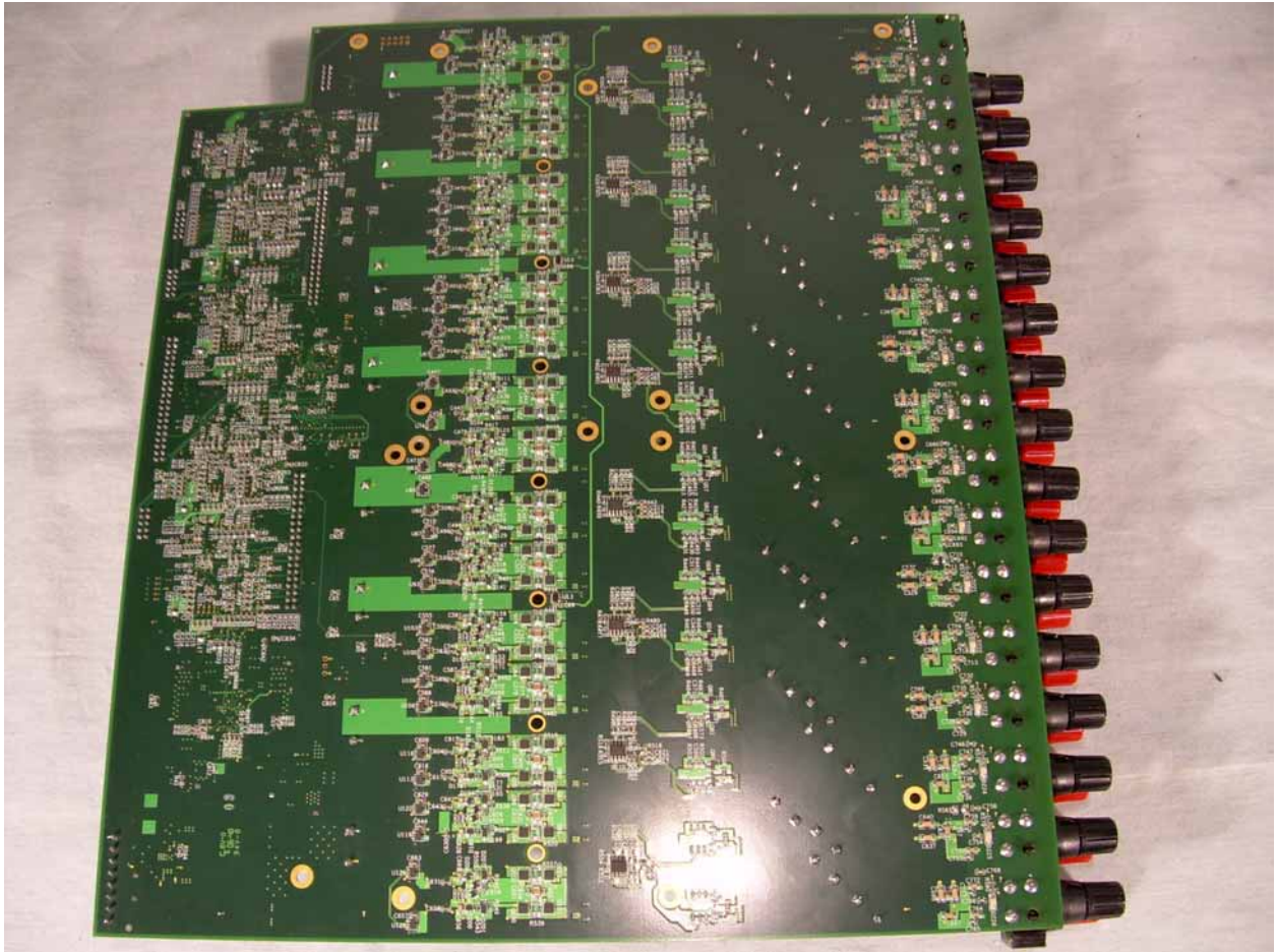
Photograph 9 - Bottom Side of the Main PCB
