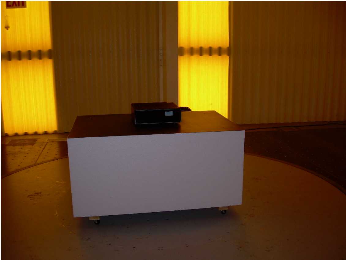
Photograph 1 - Front View Radiated Spurious Emission Test Configuration
