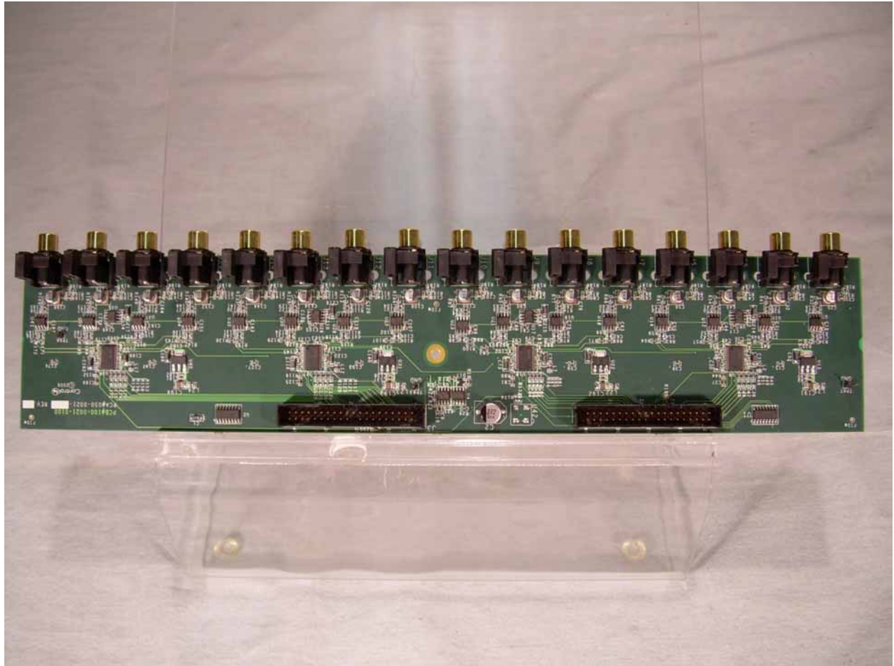
Photograph 10 - Top Side of the Rear Panel Interface PCB
