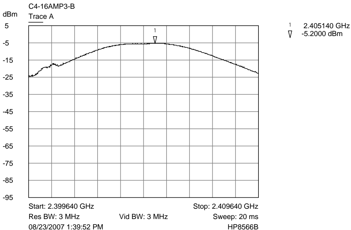
Trace A Lower channel output power plot
