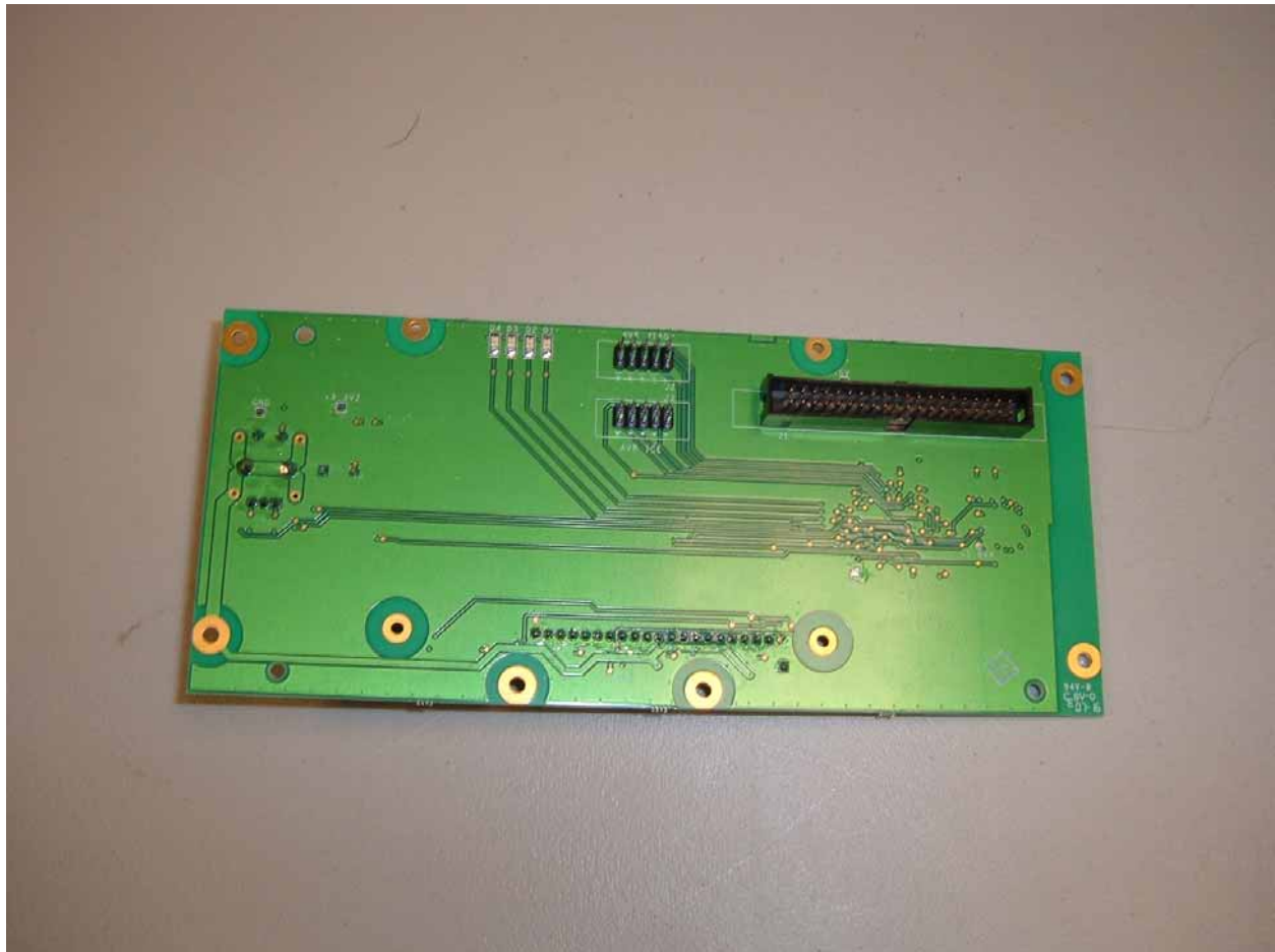
Photograph 15 - Back Side of the Front Panel PCB
