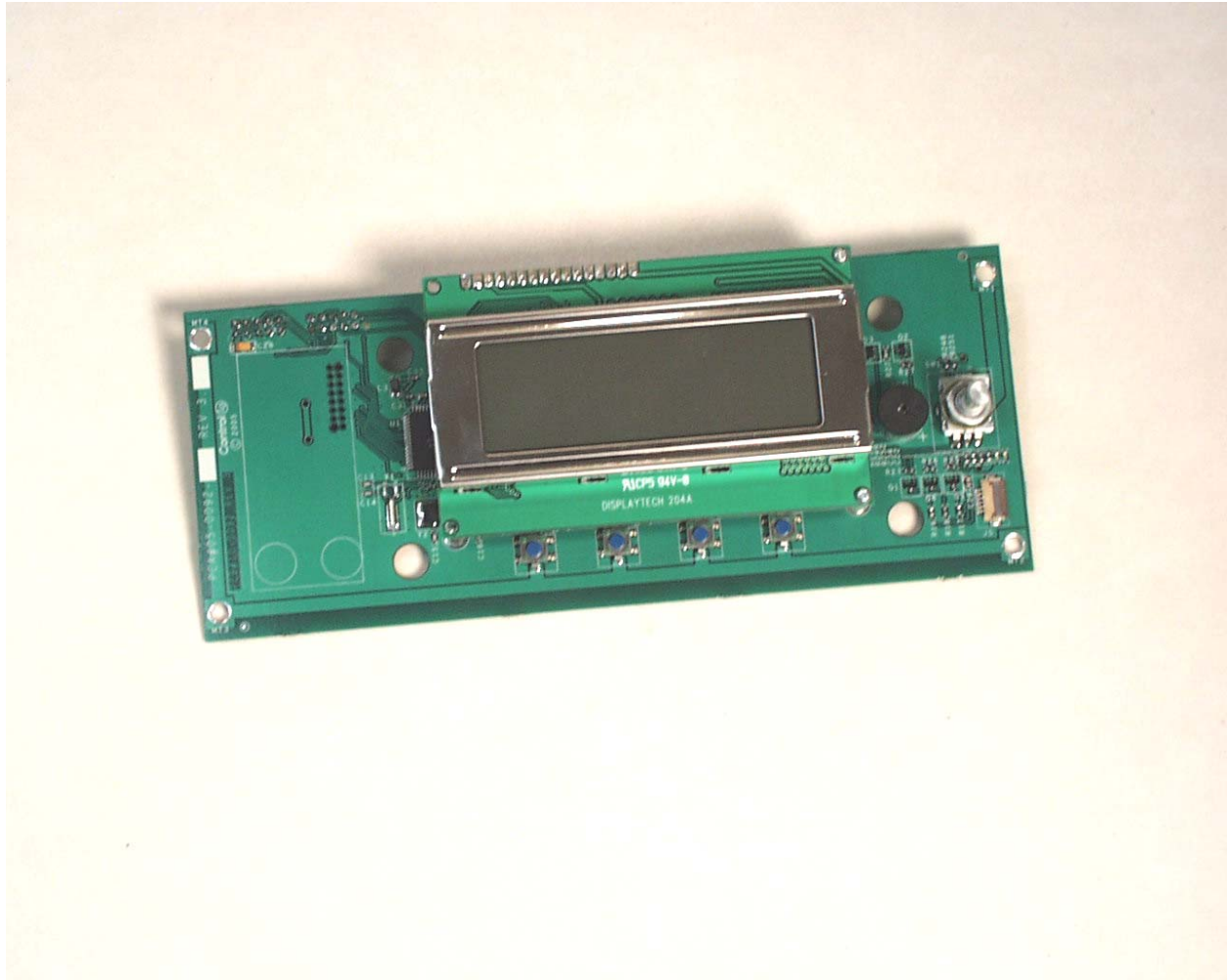
Photograph 11 - Component Side of the Front Panel PCB with Zigbee Radio Removed
