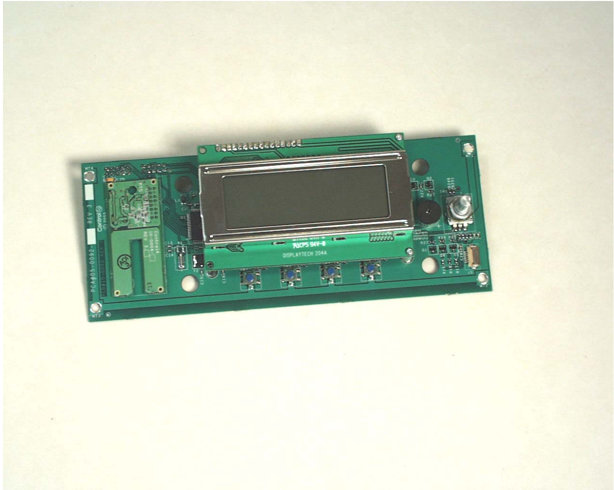
Photograph 10 - Component Side of the Front Panel PCB with Zigbee Radio
