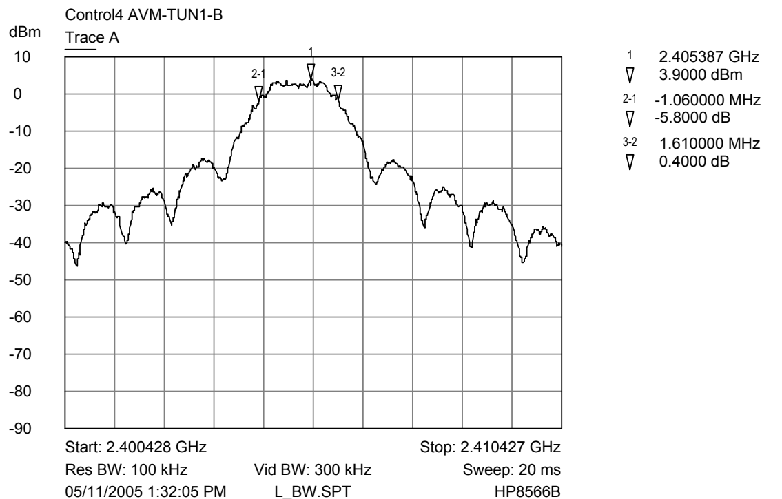
Trace A Lower Channel Bandwidth Plot
