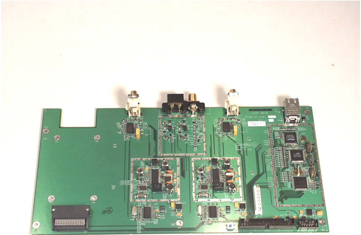
Photograph 8 - Top Side of the Main PCB
