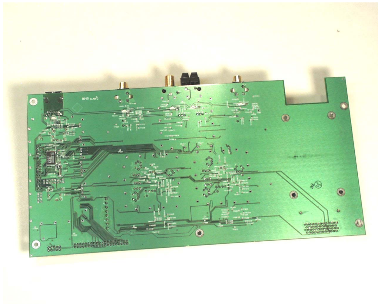
Photograph 9 - Bottom Side of the Main PCB
