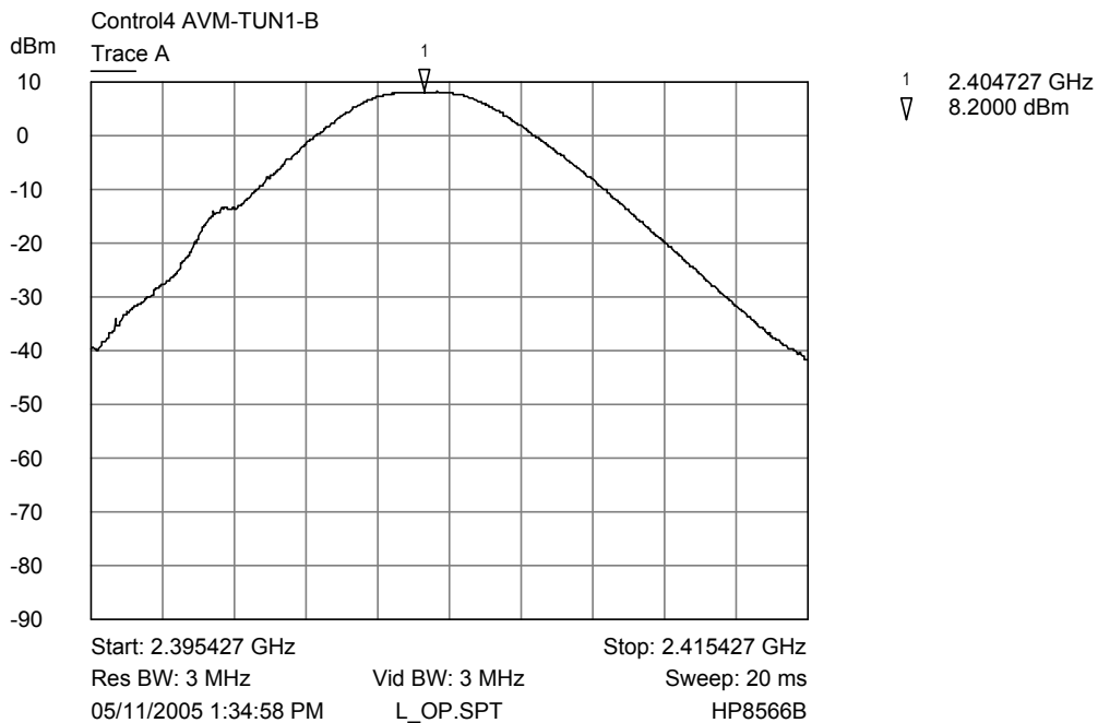
Trace A Lower Channel Output Power Plot
