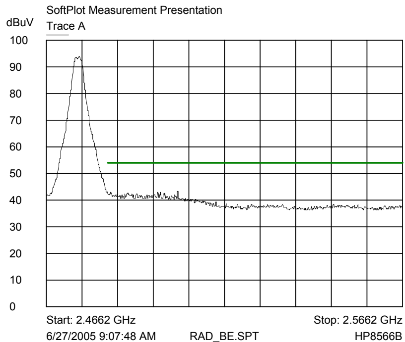
Trace A Corrected upper band edge plot
