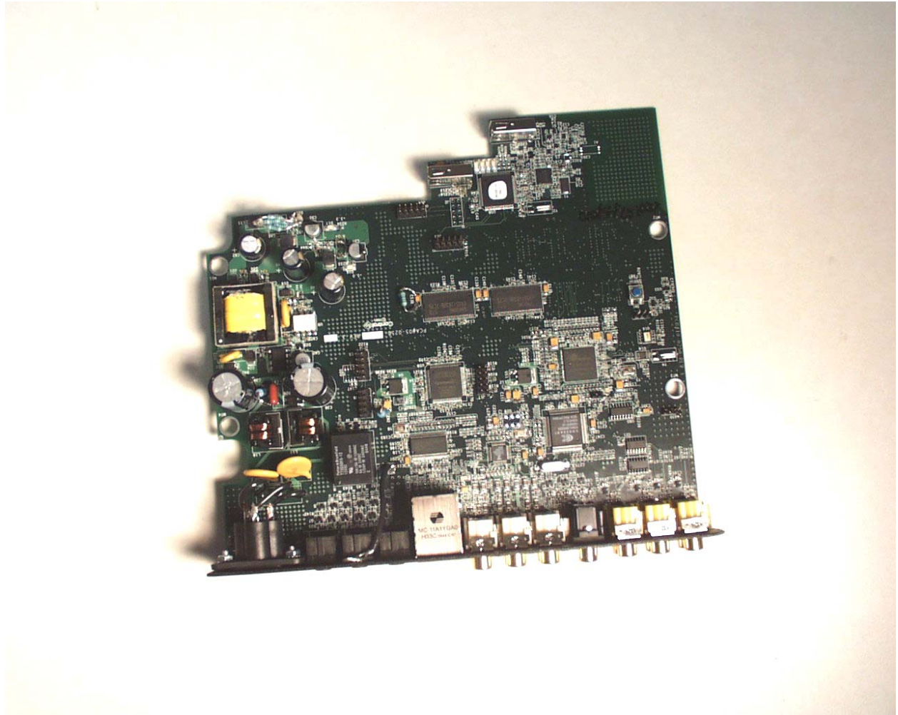
Photograph 8 - View of the Main PCB without the USB Devices Installed
