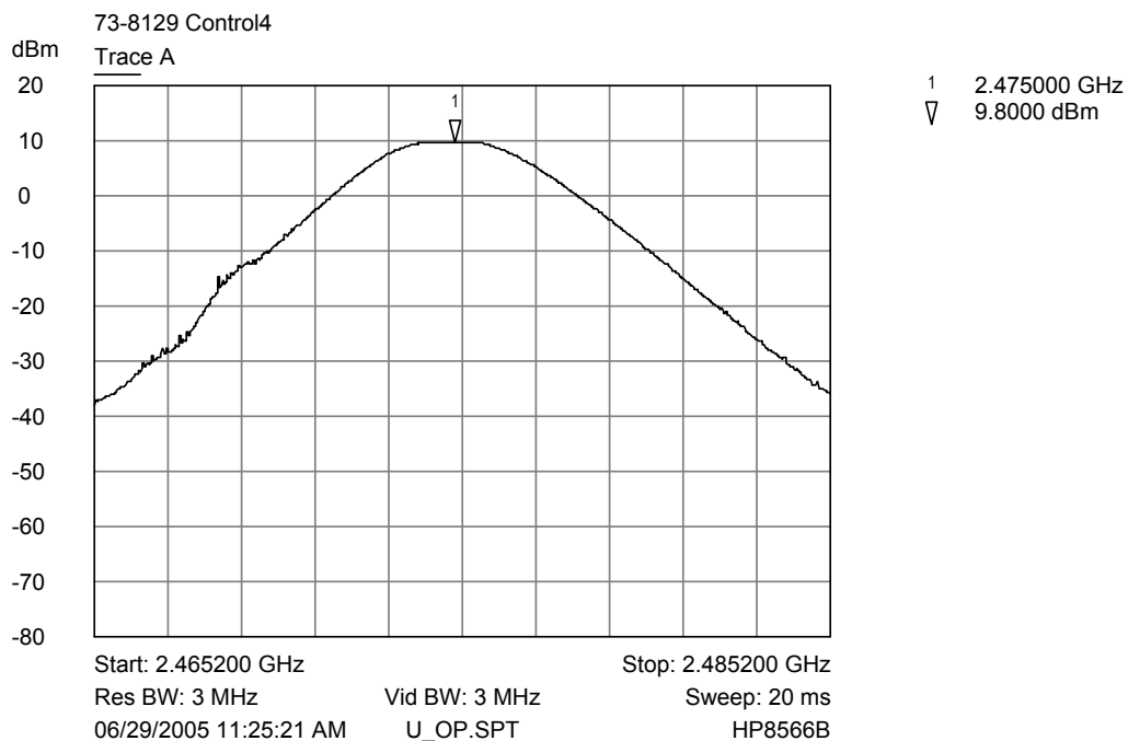
Trace A Upper Channel Output Power Plot
