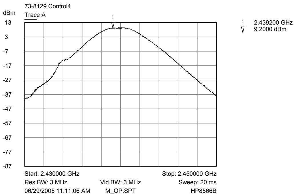
Trace A Middle Channel Output Power Plot
