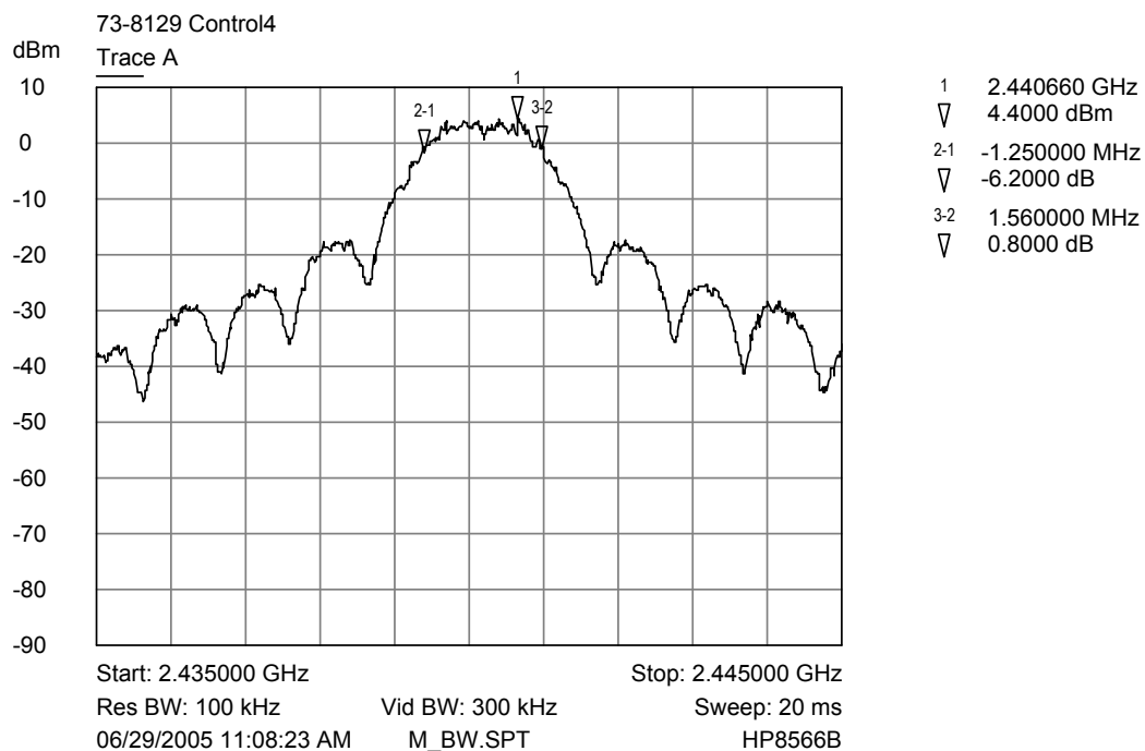
Trace A Middle Channel Bandwidth Plot
