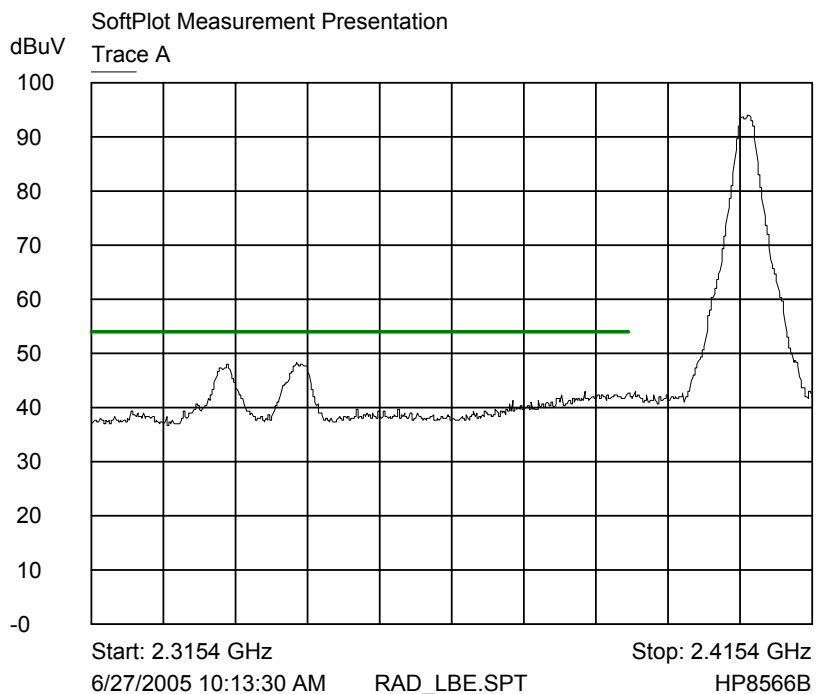
Trace A Corrected lower band edge plot
