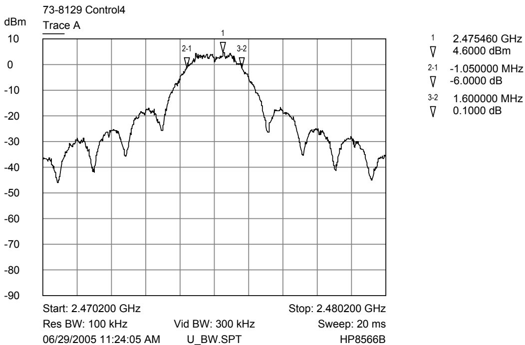
Trace A Upper Channel Bandwidth Plot
