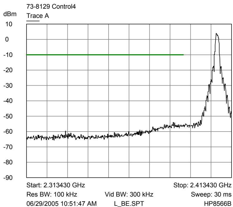
Trace A Lower Channel Band Edge
