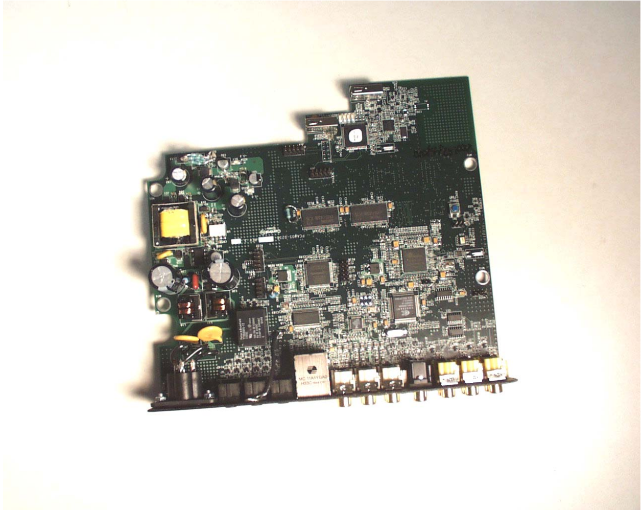
View of the Main PCB without the USB Devices Installed
