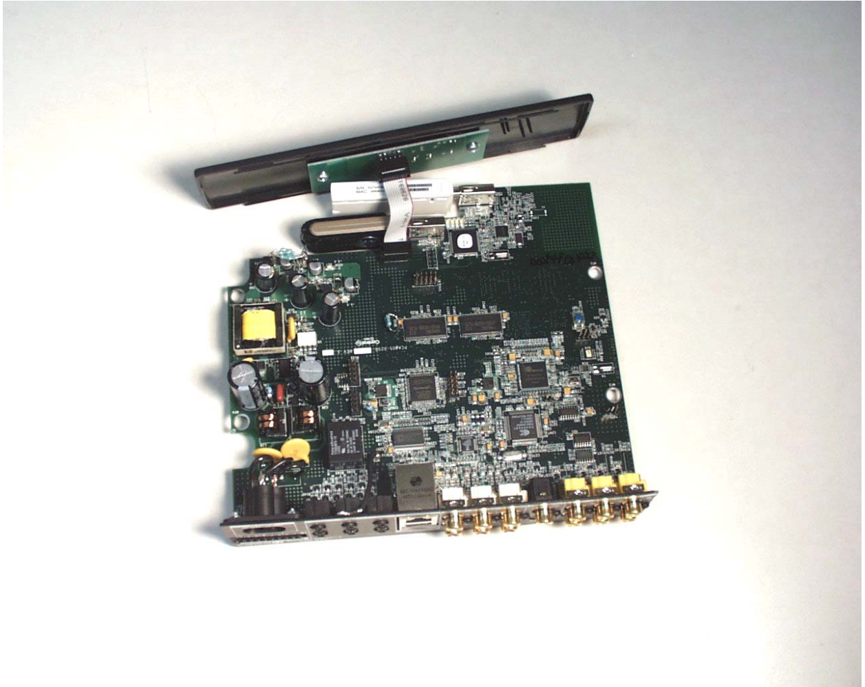
Internal View of the EUT with the USB Devices Installed
