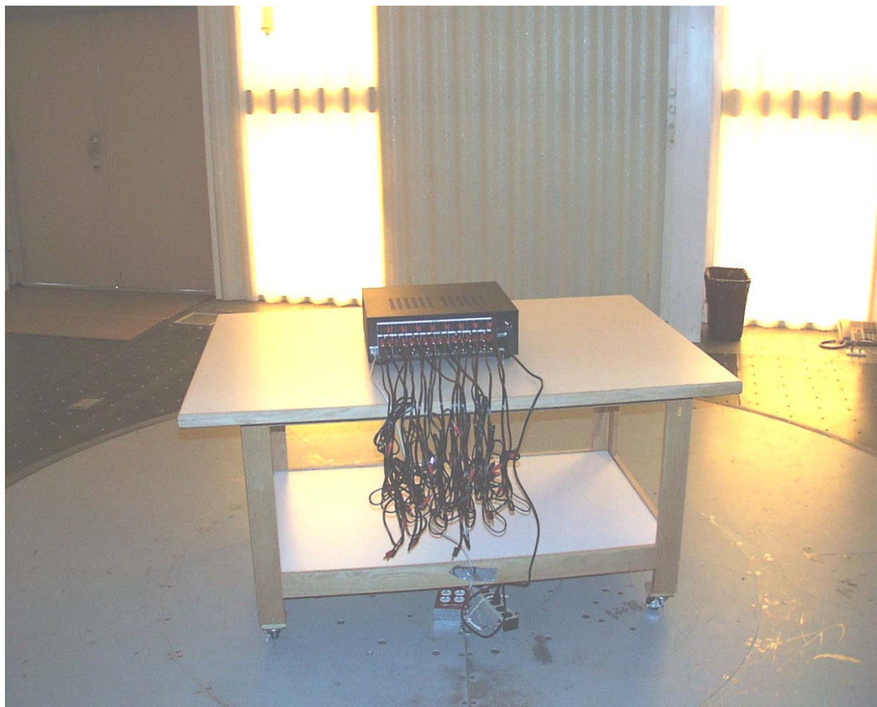
Photograph 2 - Back View Radiated Disturbance Worst Case Configuration
