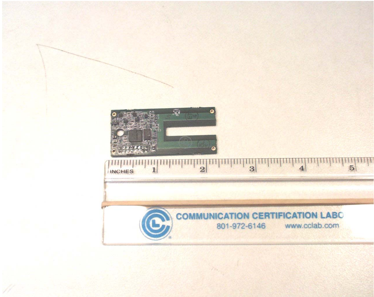
Photograph 7 - Component Side of the Transceiver PCB
