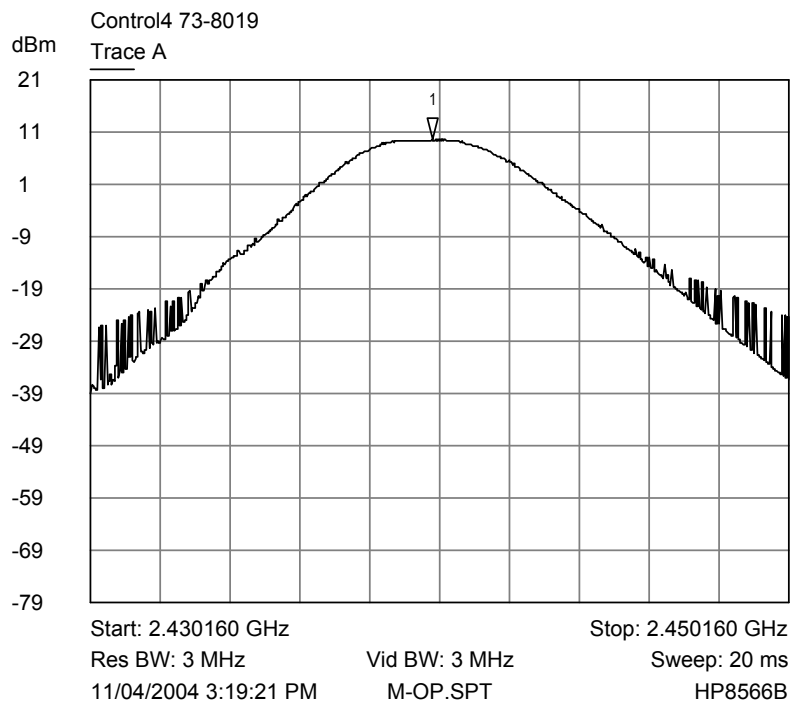
Trace A Middle Channel Output Power
