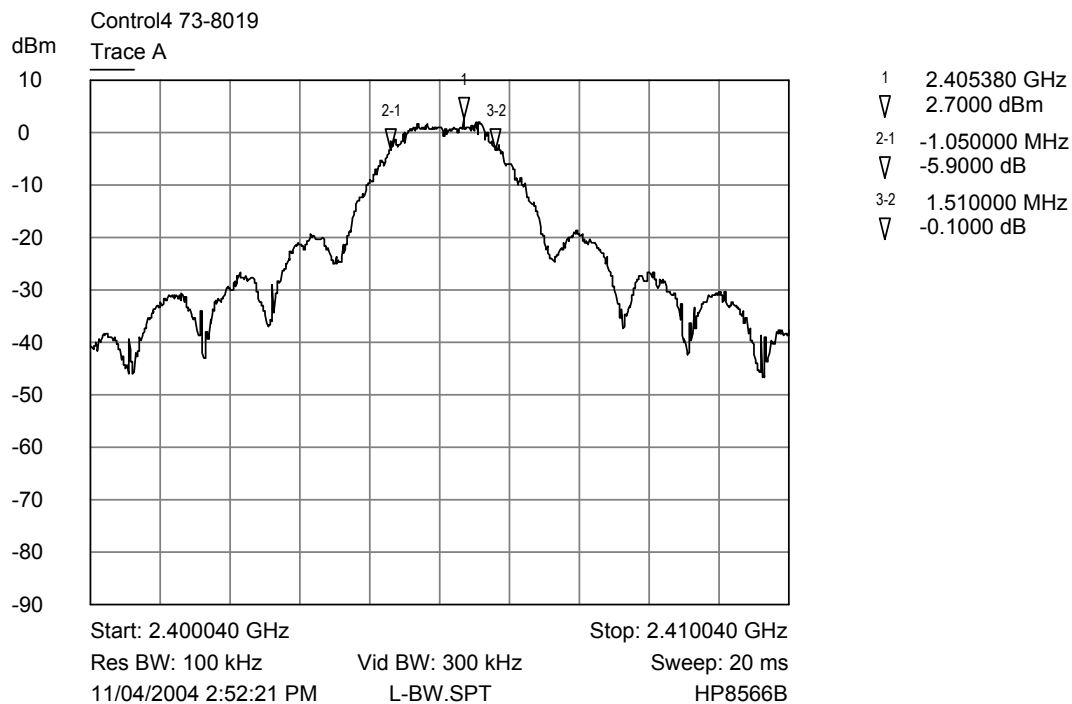
Trace A Lower channel bandwidth
