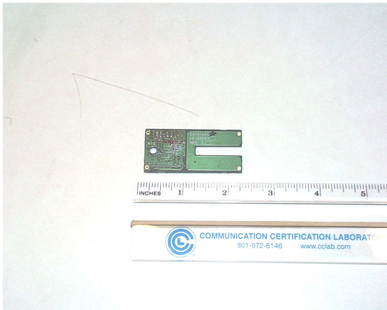
Photograph 6 - Trace Side of Transceiver PCB
