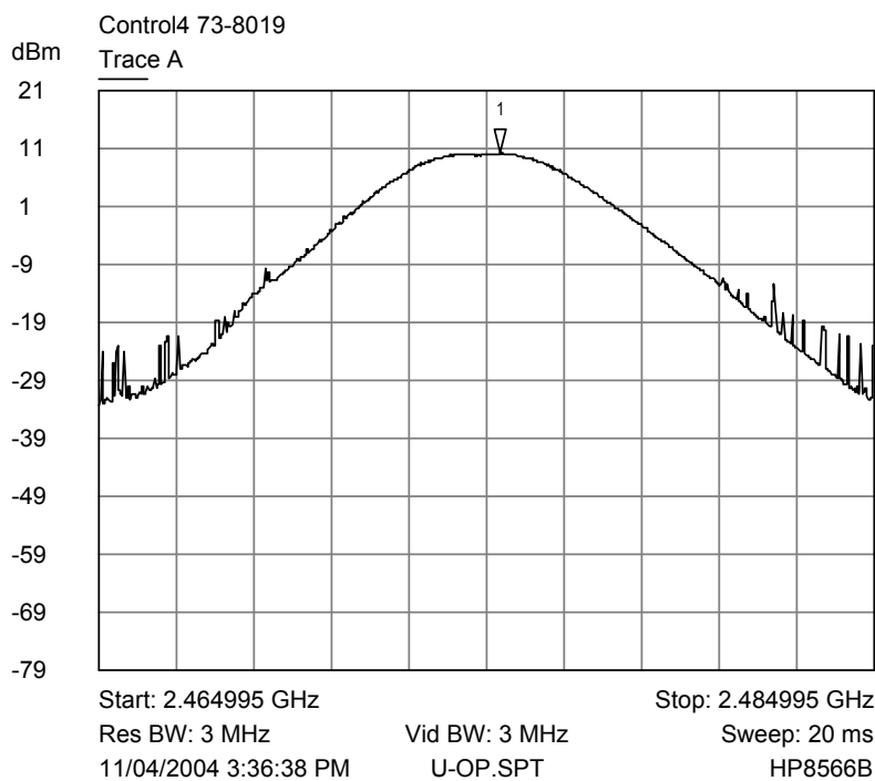
Trace A Upper channel Output Power
