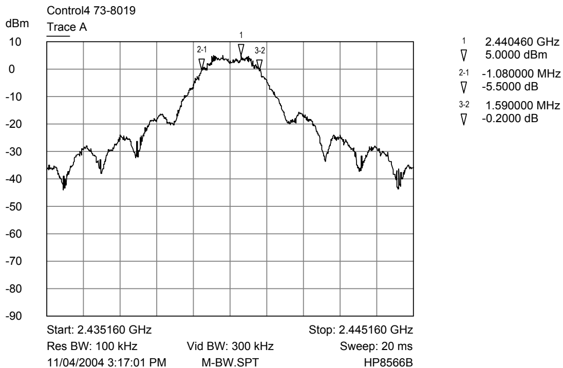
Trace A Middle Channel Bandwidth
