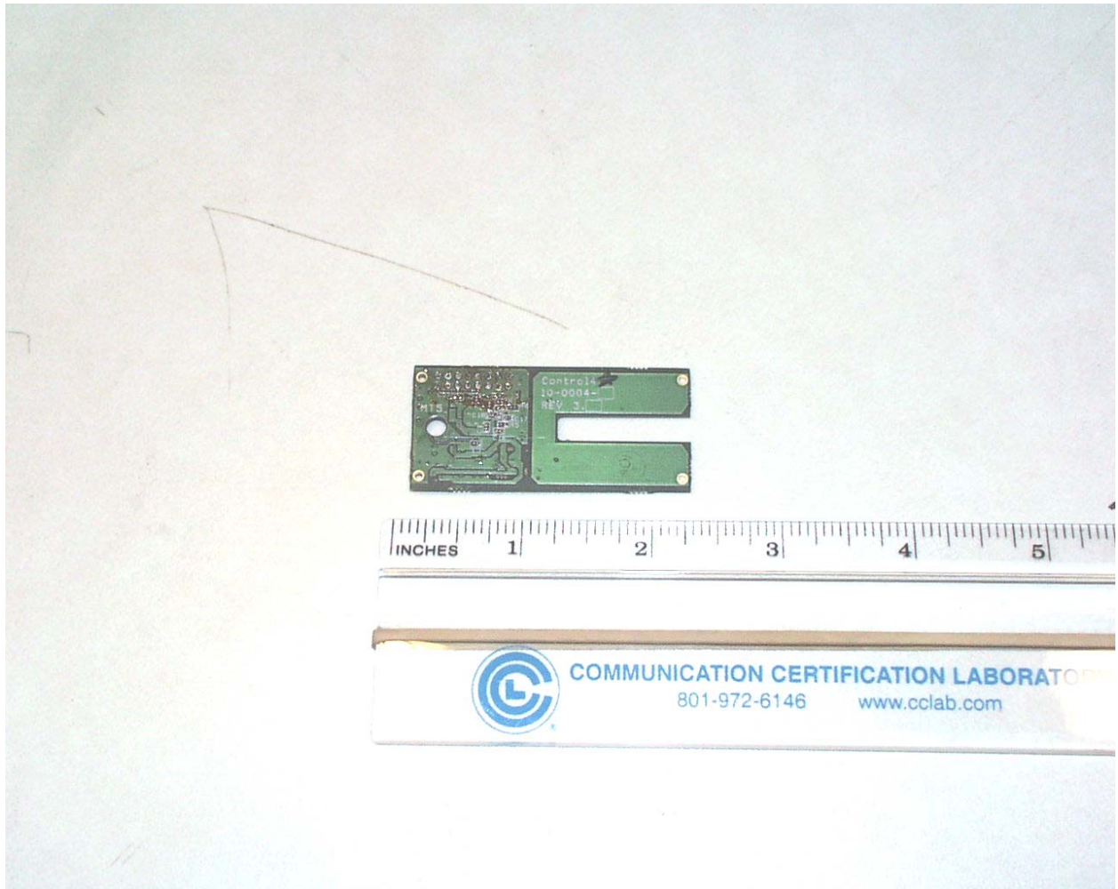
Trace Side of Transceiver PCB
