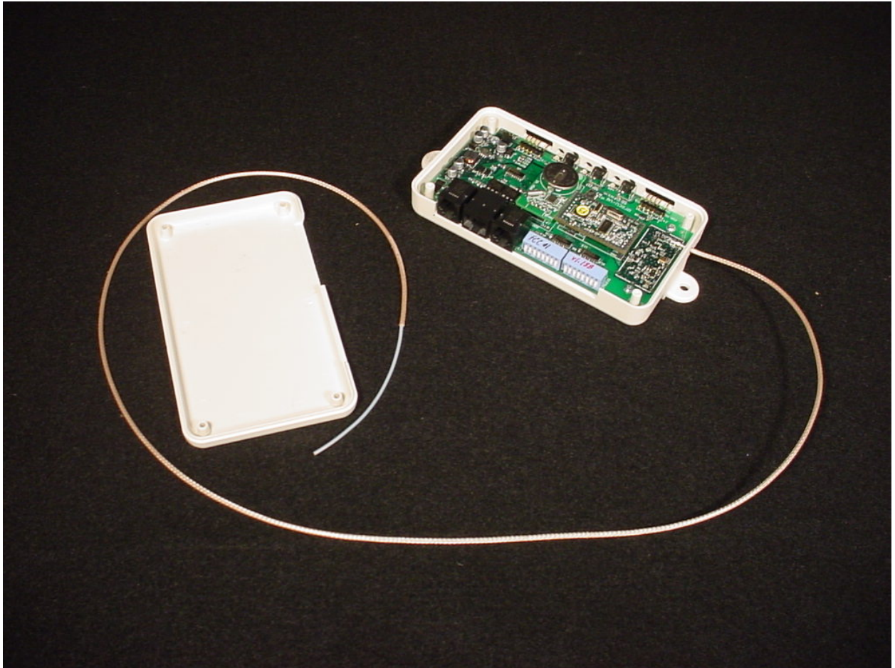
Figure 1: Internal View
