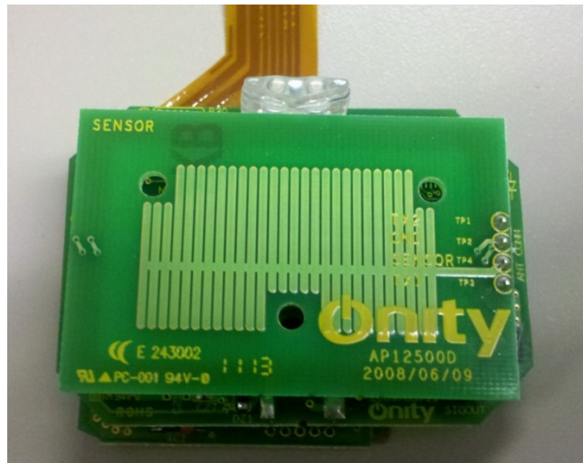
Photo of EUT Antenna
