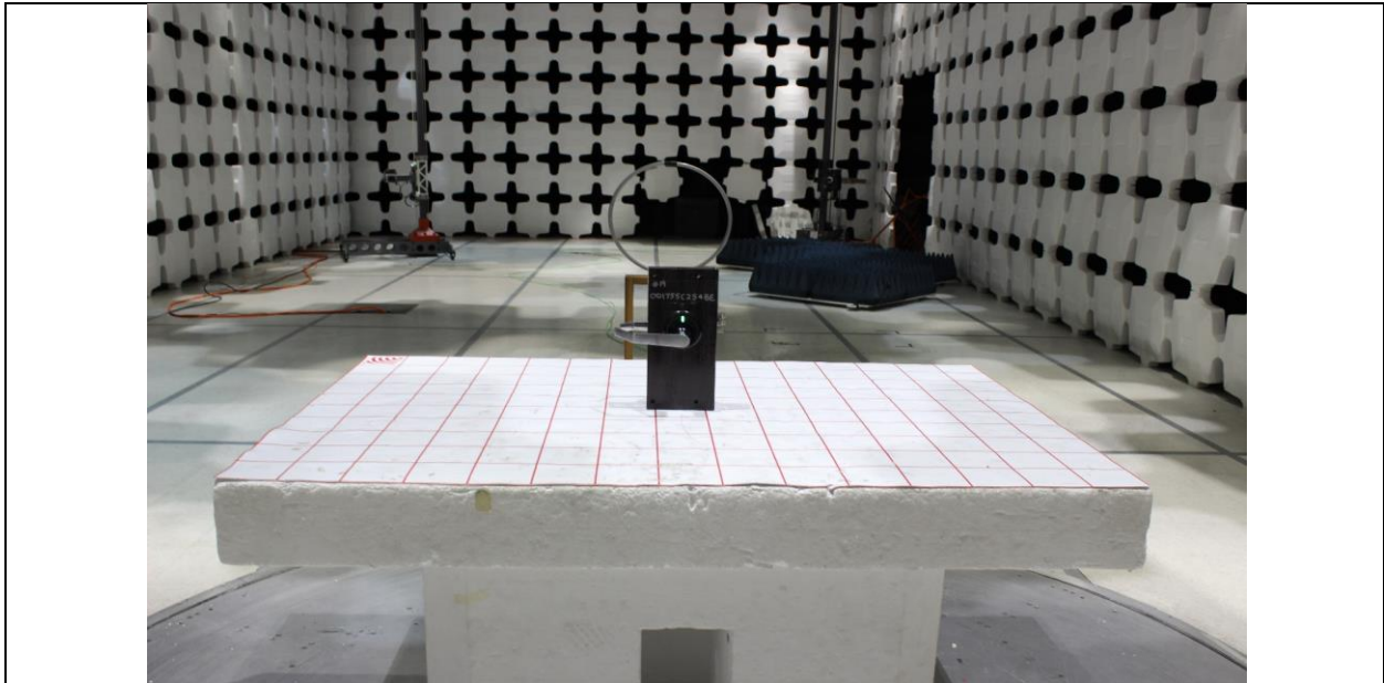
Radiated Emission Test Below 30MHz Front View
