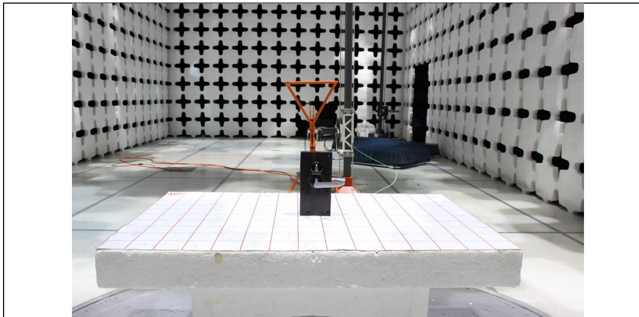
Radiated Emission Test Below 1GHz Front View
