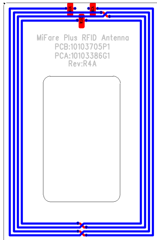
Right – PCB Layout of Antenna
