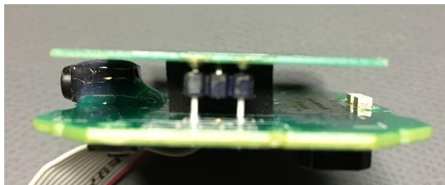
Figure 3. Connection between RFID antenna PCB and RFID reader PCB
