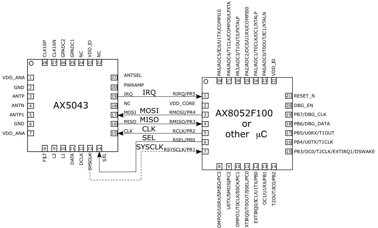
Figure 2. Connecting AX5043 to AX8052F100 or other \mu C
