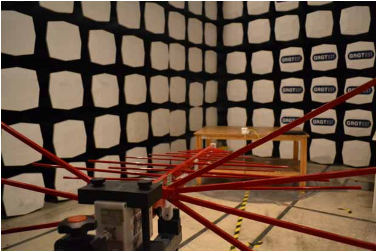
Radiated Emission
