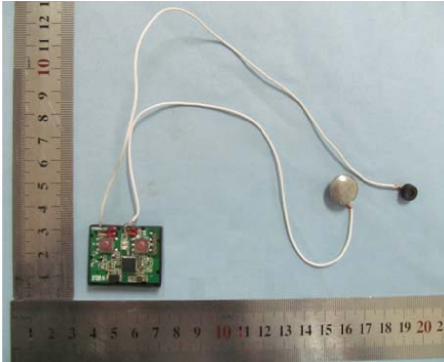
FRONT VIEW OF PCB
