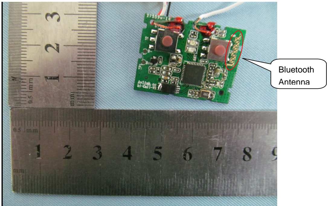
FRONT VIEW OF PCB
