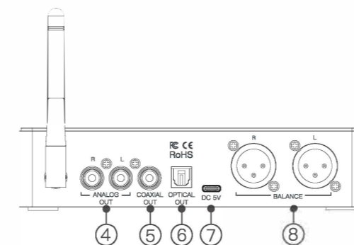
Rear Panel
