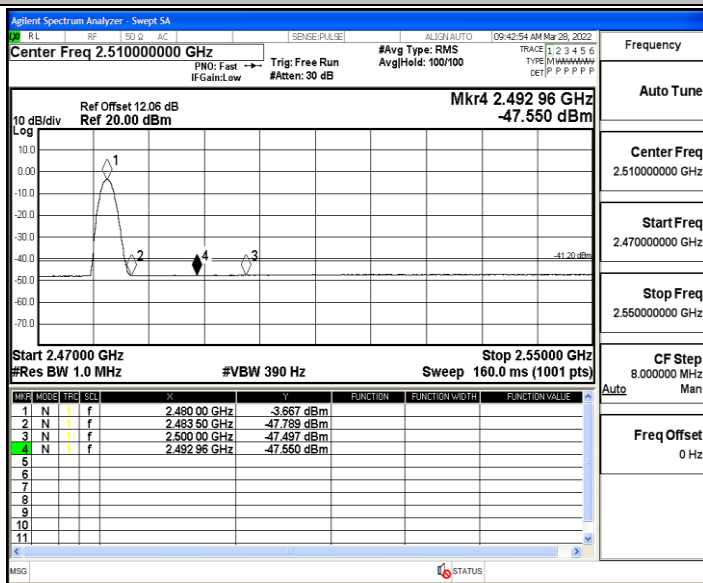
2DH5_Ant1_High_2480_Peak
