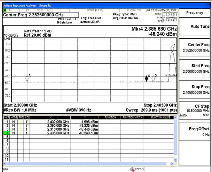
2DH5_Ant1_Low_2402_Peak
