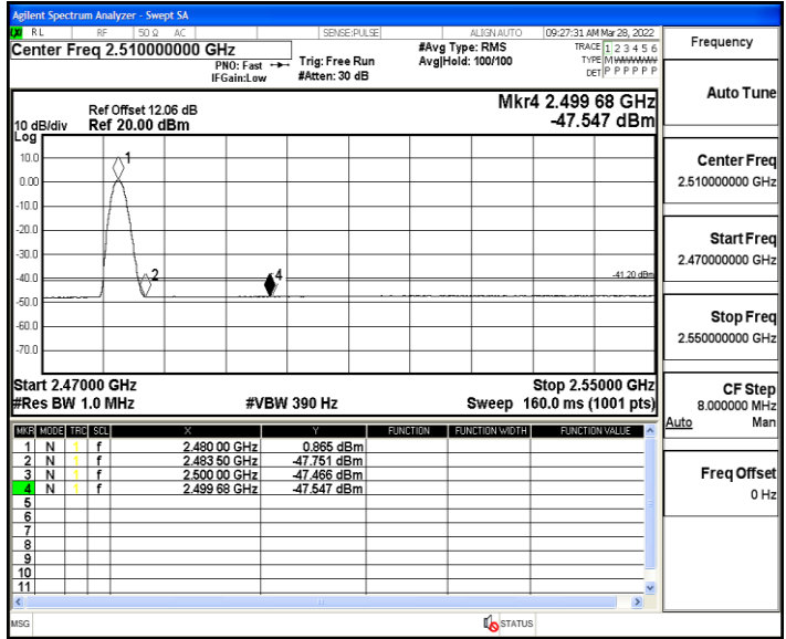
DH5_Ant1_High_2480_Peak
