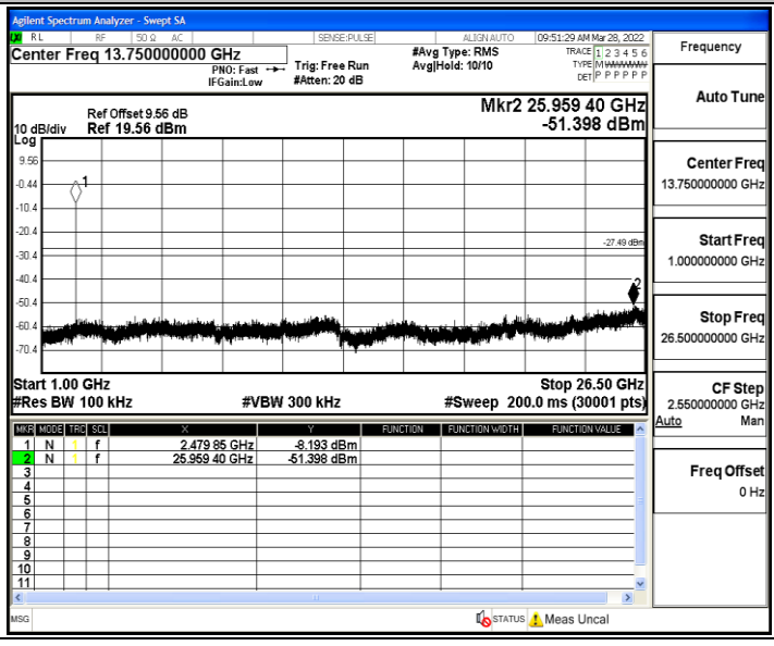
3DH5_Ant1_2480_1000~26500
