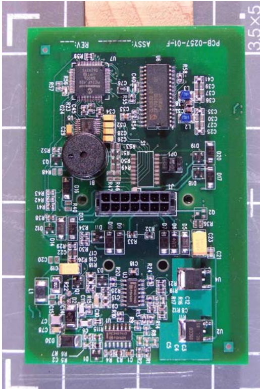
XF1560CS2 – PCB Back
