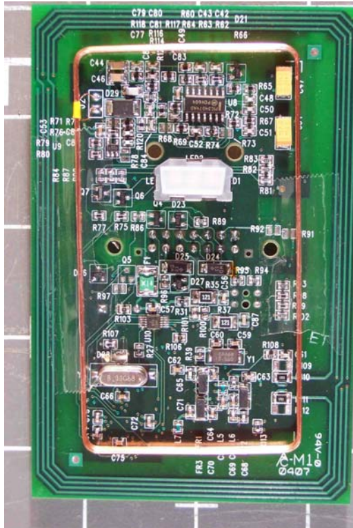
XF1560CS4 – PCB Front
