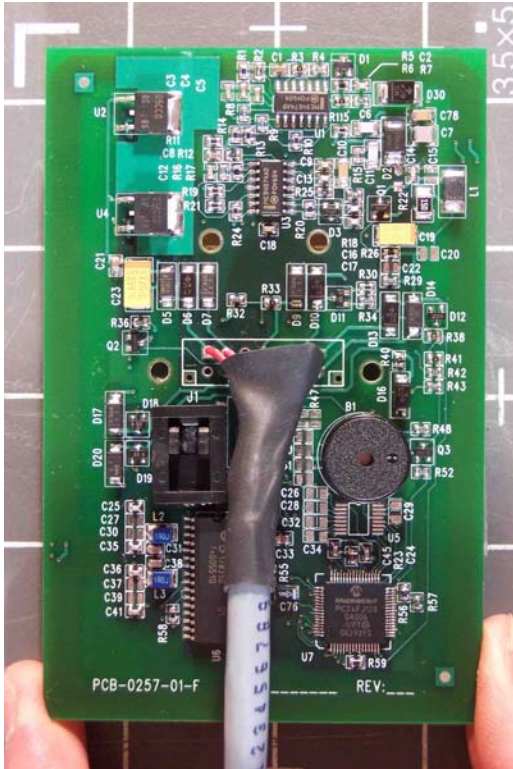
XF1500P – PCB Back 2
