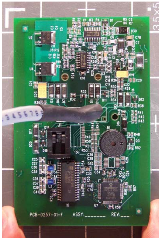
XF1500P – PCB Back 1
