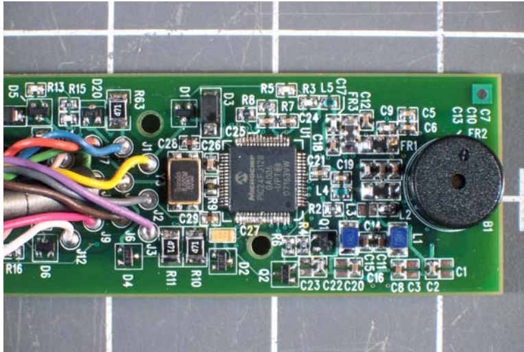
PCB bk closeup 2
