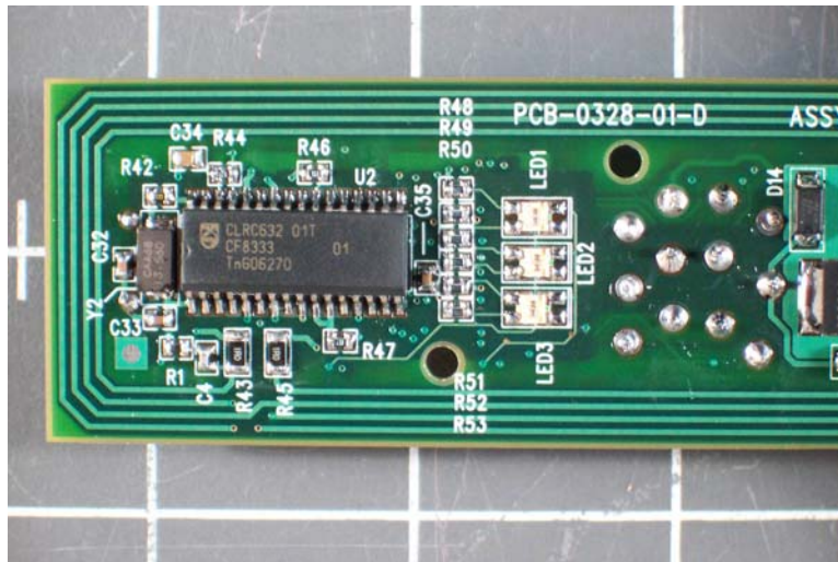
PCB fr closeup 1
