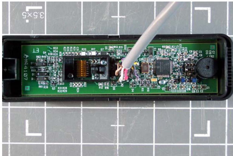
Int bk without potting
