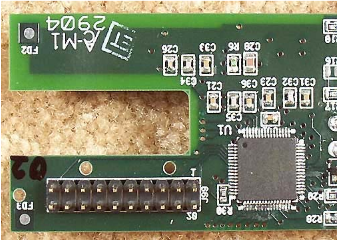
Base Back PCB Close-up 1
