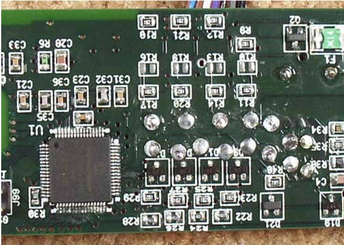
Base Back PCB Close-up 2
