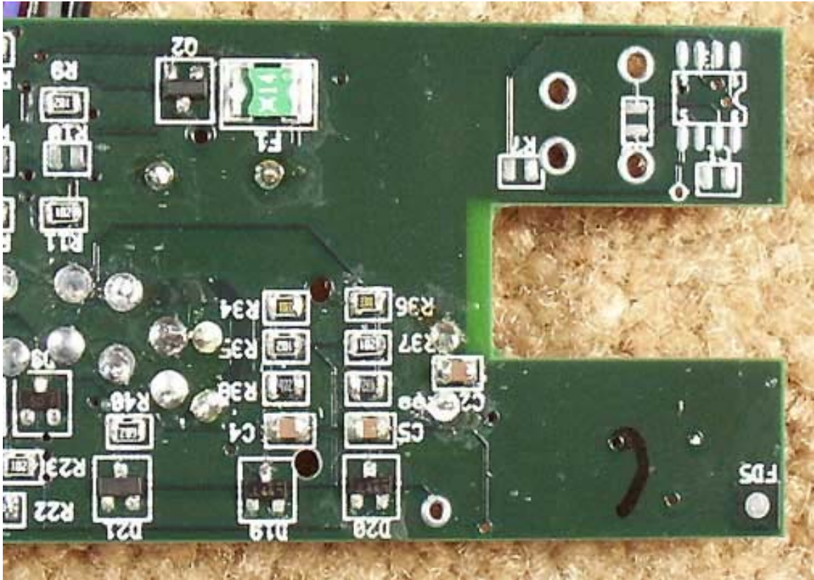
Base Back PCB Close-up 3
