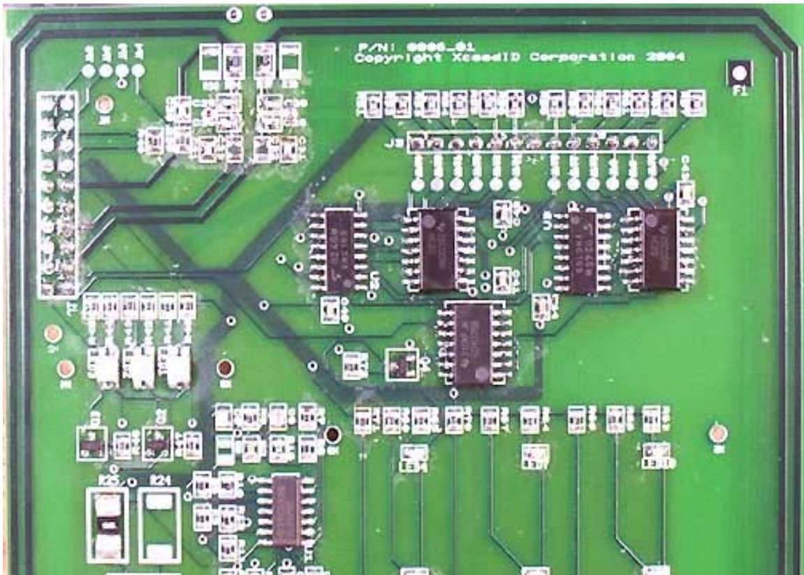
21xx Front Antenna PCB Close-up 3
