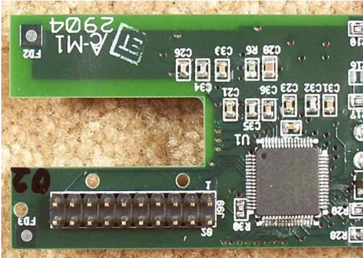
Base PCB Back Close-up 1
