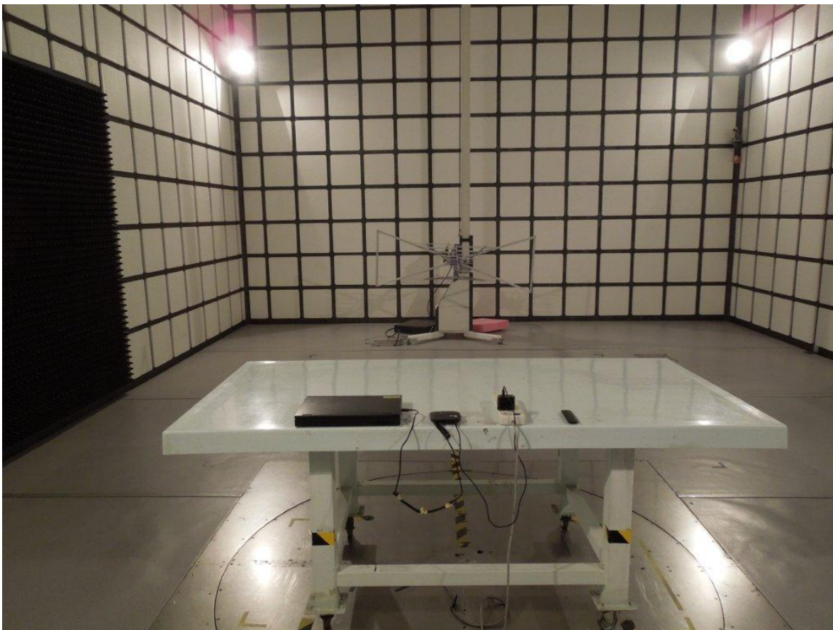
Radiated Emission (30MHz -1GHz) Setup photo
