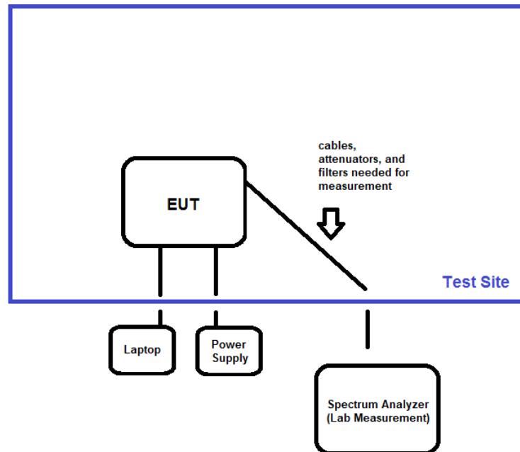
Test Setup Block Diagram (Conducted)
