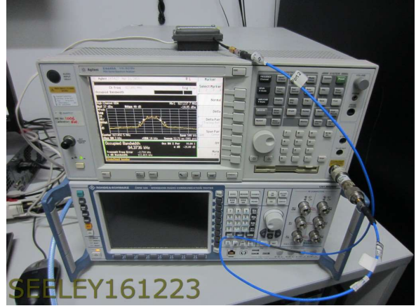
Antenna Port Tests – Wireless Receiver
