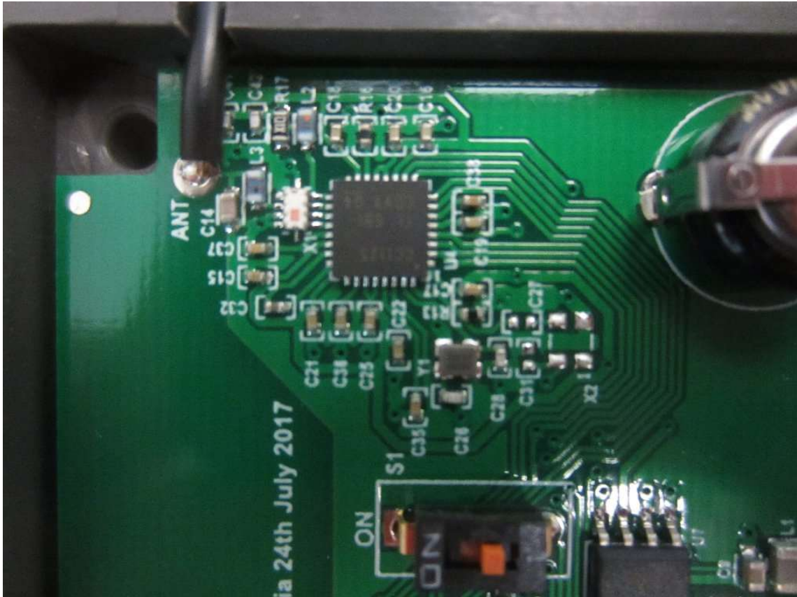
Wireless Receiver PCB (Transceiver Circuit)
