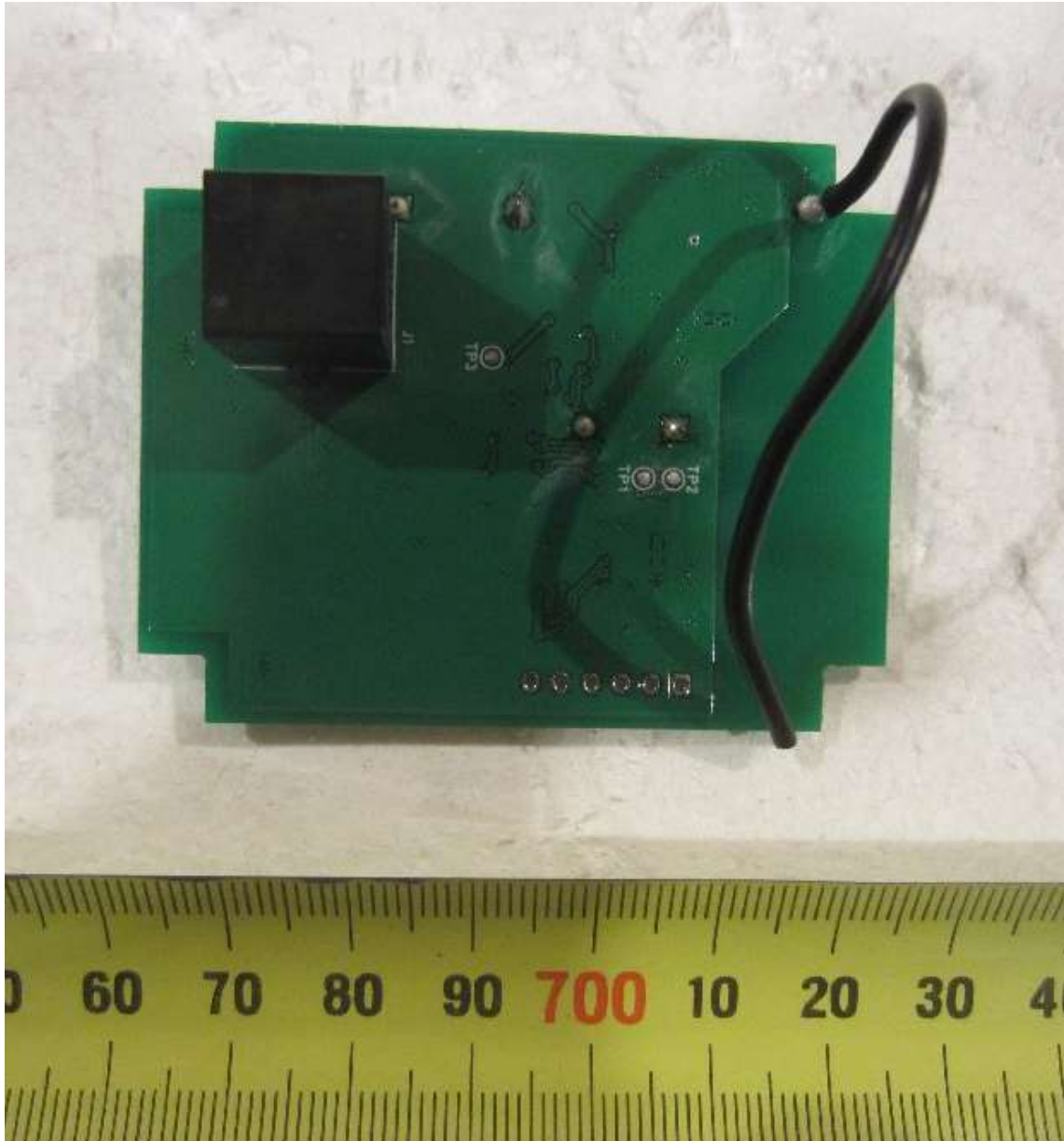
Wireless Receiver PCB (Trace Side)
