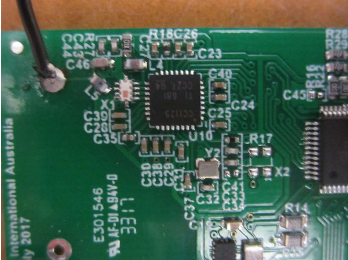
Wireless Smart Controller PCB (Transceiver Circuit)
