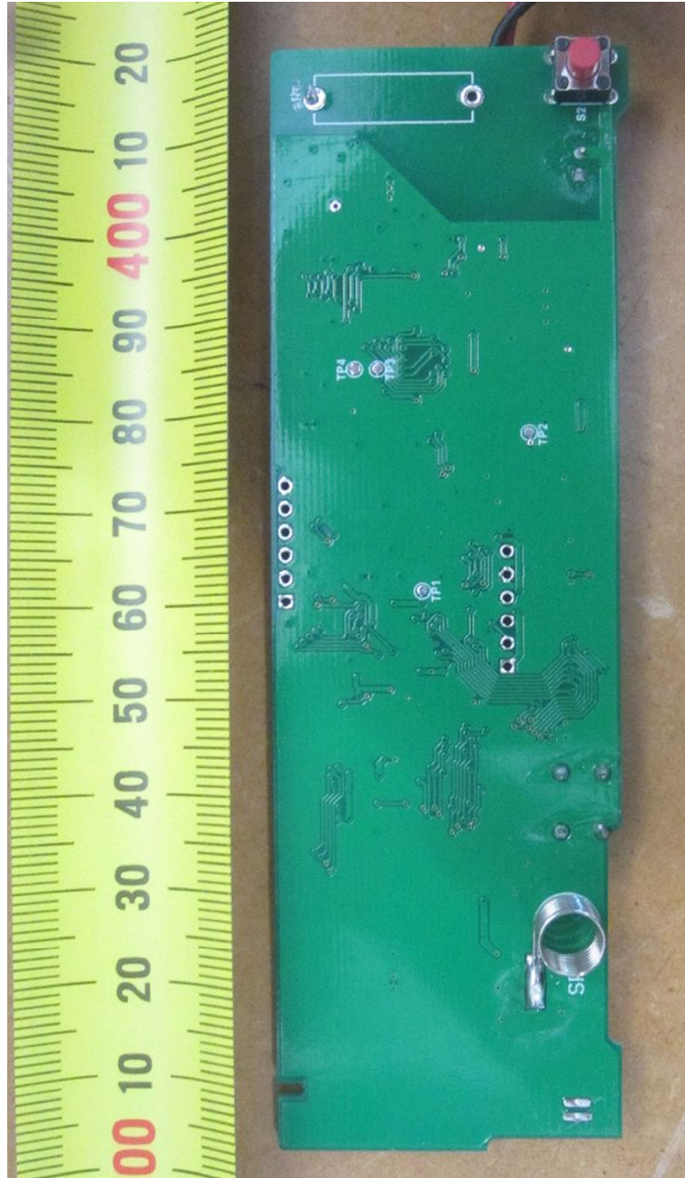
Wireless Smart Controller PCB (Trace Side)
