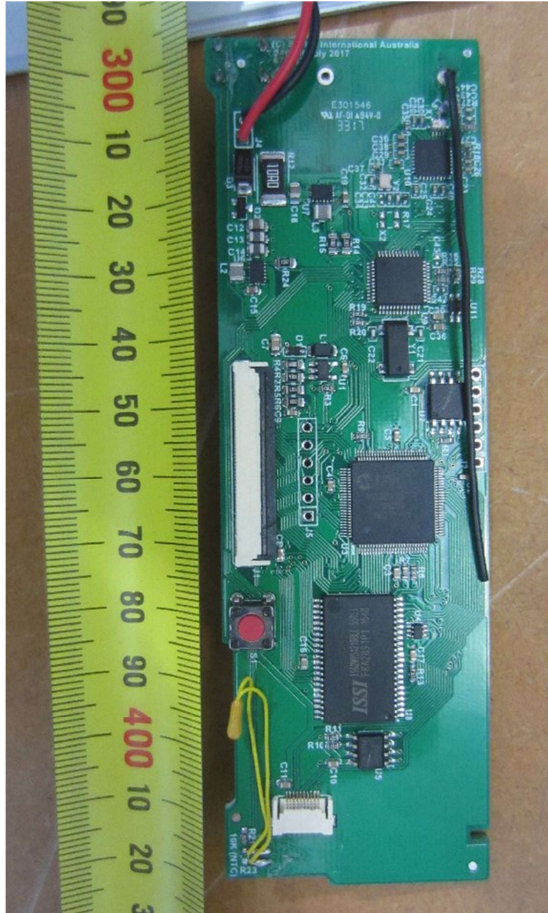
Wireless Smart Controller PCB (Component Side)
