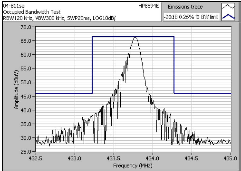
Figure 1: Breezair Freedom emitted spectrum (max hold)
