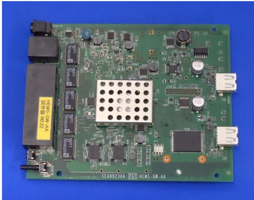
Main PCB Top Side
