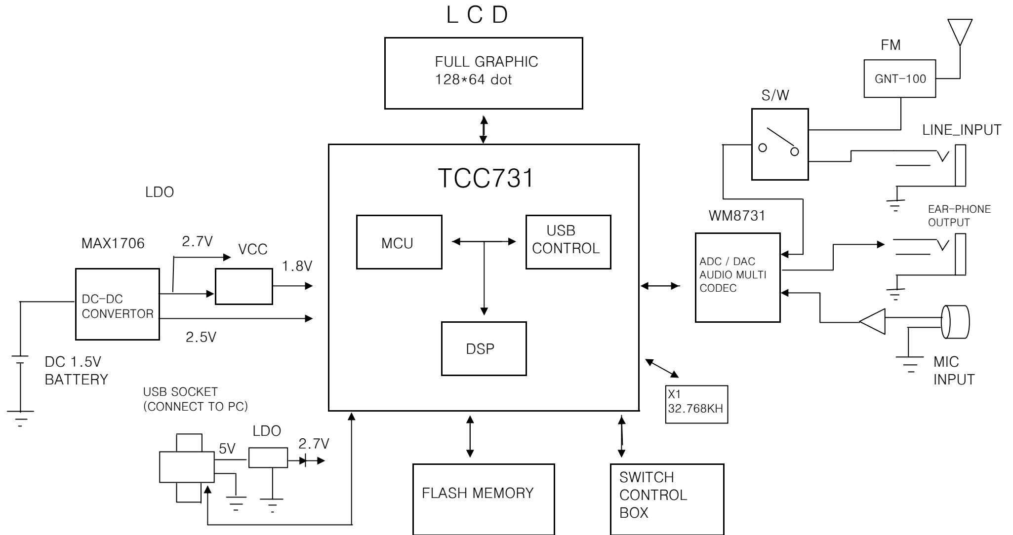
FXA-1560 BLOCK DIAGRAM
