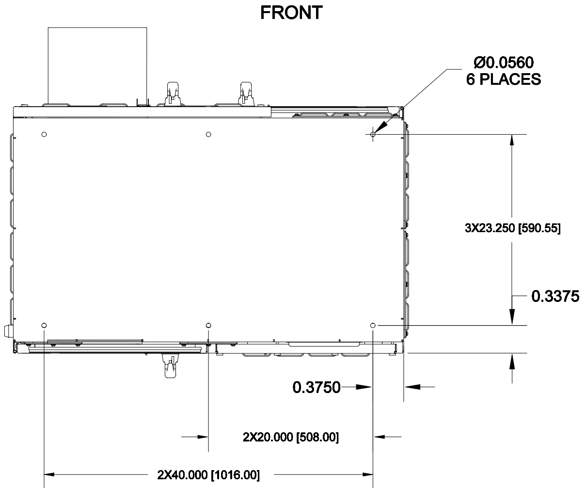
Figure 2.2 Clearance Holes in RadioRouter Base — Bottom View
