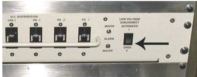
Figure 7.4 Low Voltage Disconnect
