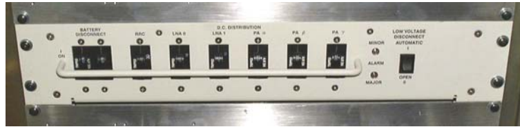
Figure 7.2 DC Power Distribution Panel — Front View
