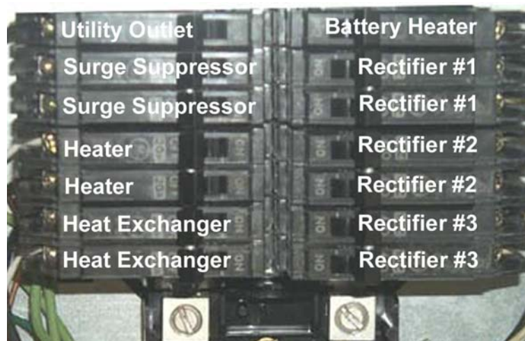
Figure 7.3 Turning AC Breakers On
