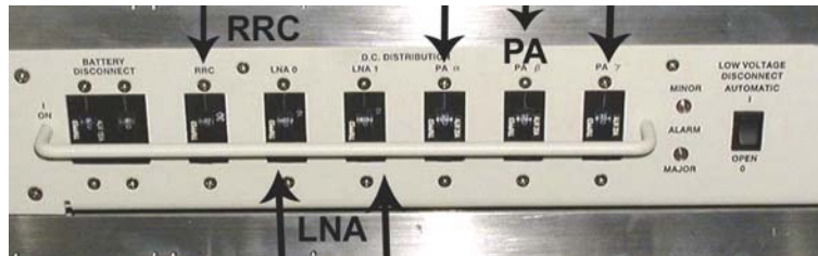
Figure 7.6 DC Circuit Breakers
