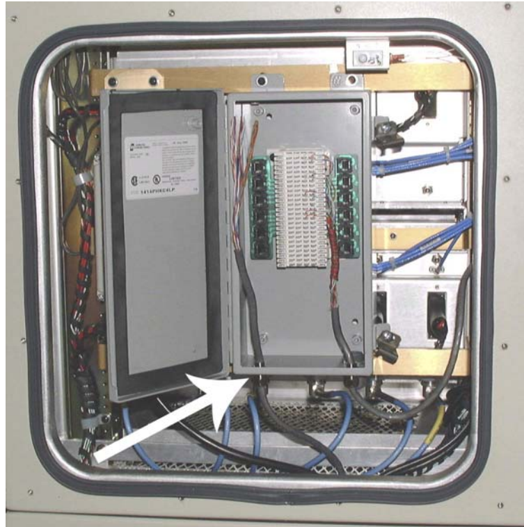
Figure 5.4 T1 Termination Box Open
