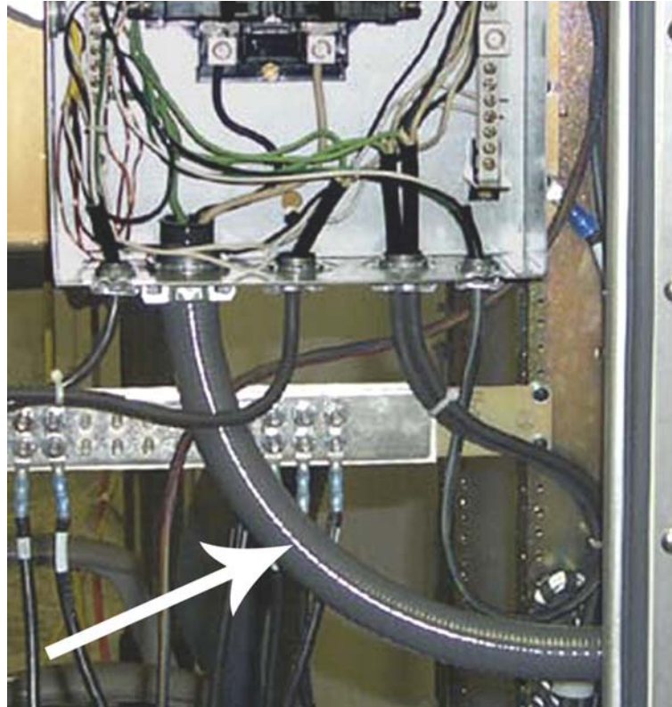
Figure 4.2 Path of Power Cable to AC Load Center — Rear View
