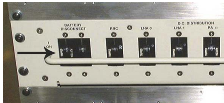
Figure 7.5 DC Battery Breakers
