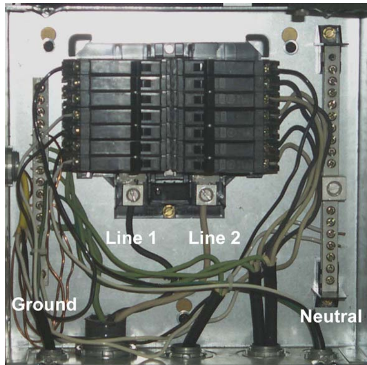
Figure 4.3 Load Center Connections
