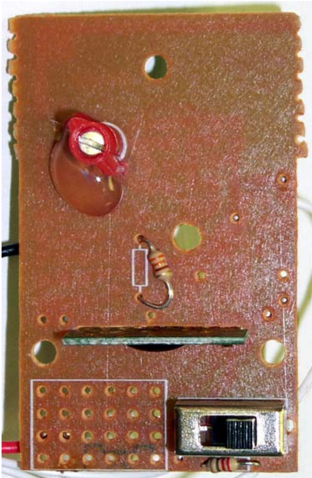
Component Side
