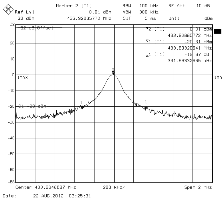
Emission Bandwidth
