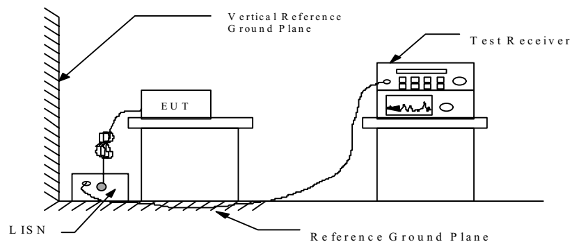
Figure 3 : Conducted emissions measurement configuration
