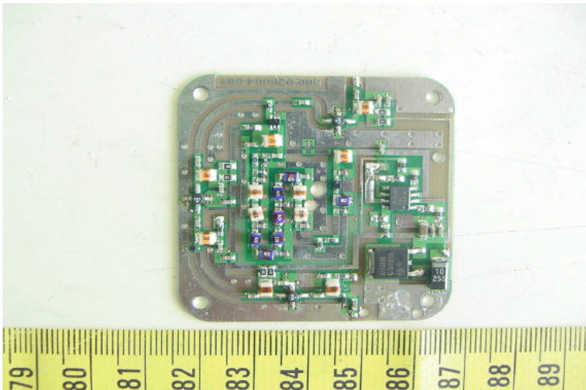
54. Component View of PCB 6
