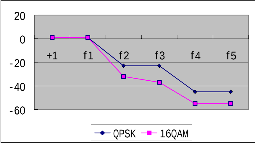
Example of the transmitting spectrum
