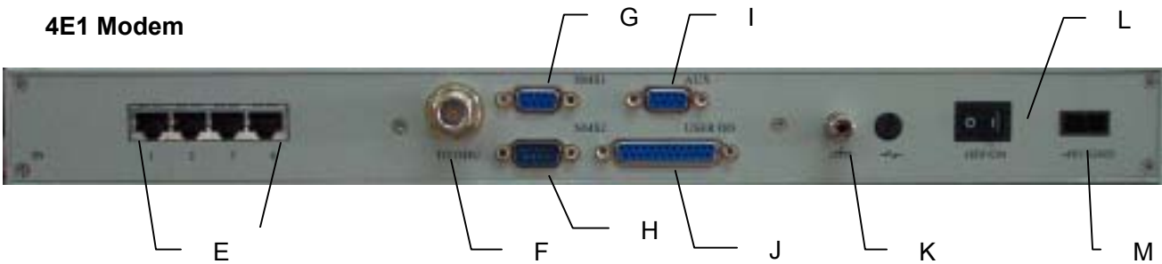
Rear Panel
