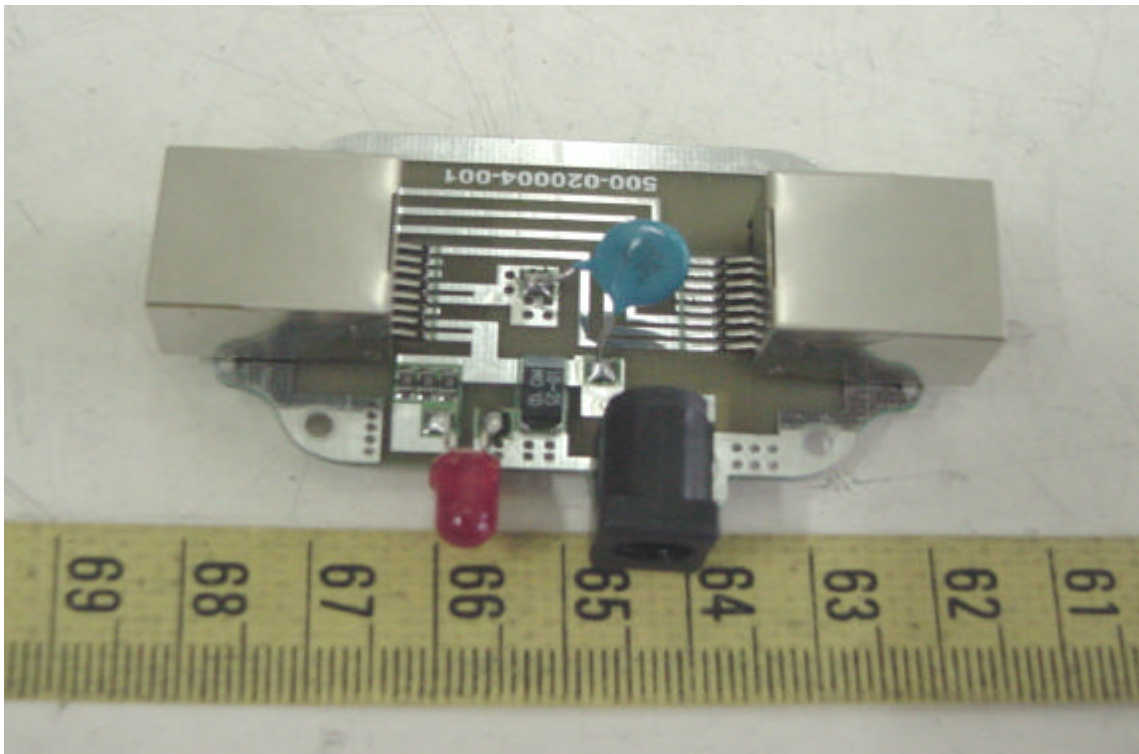
Component View of POE's PCB
