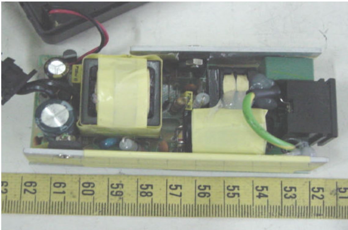
Component View of Power Adaptor's PCB
