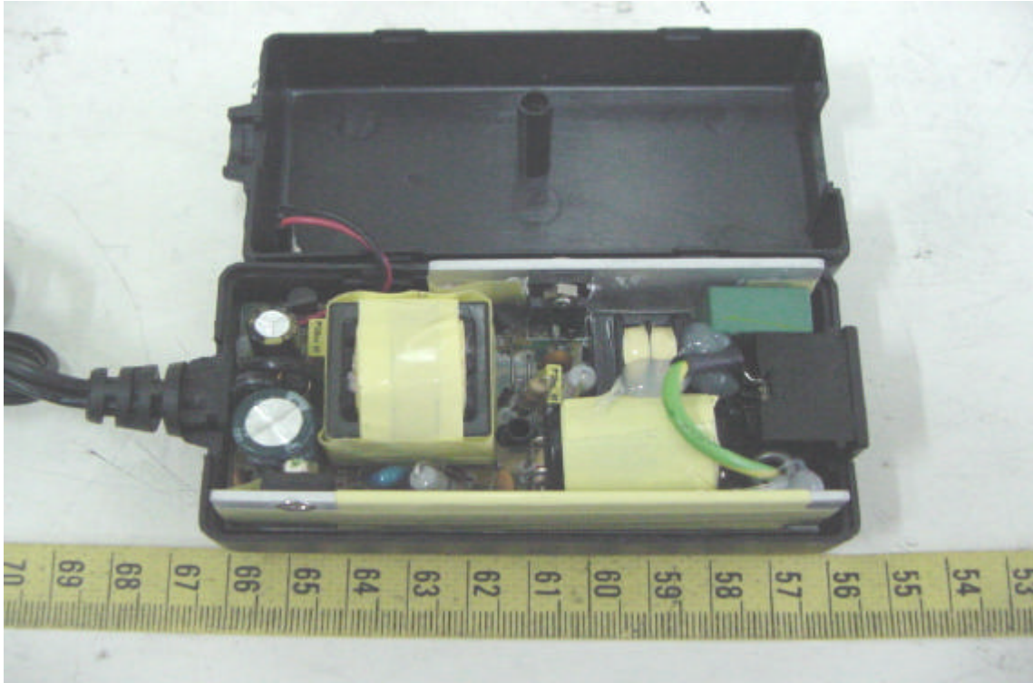
Internal View of Power Adaptor
