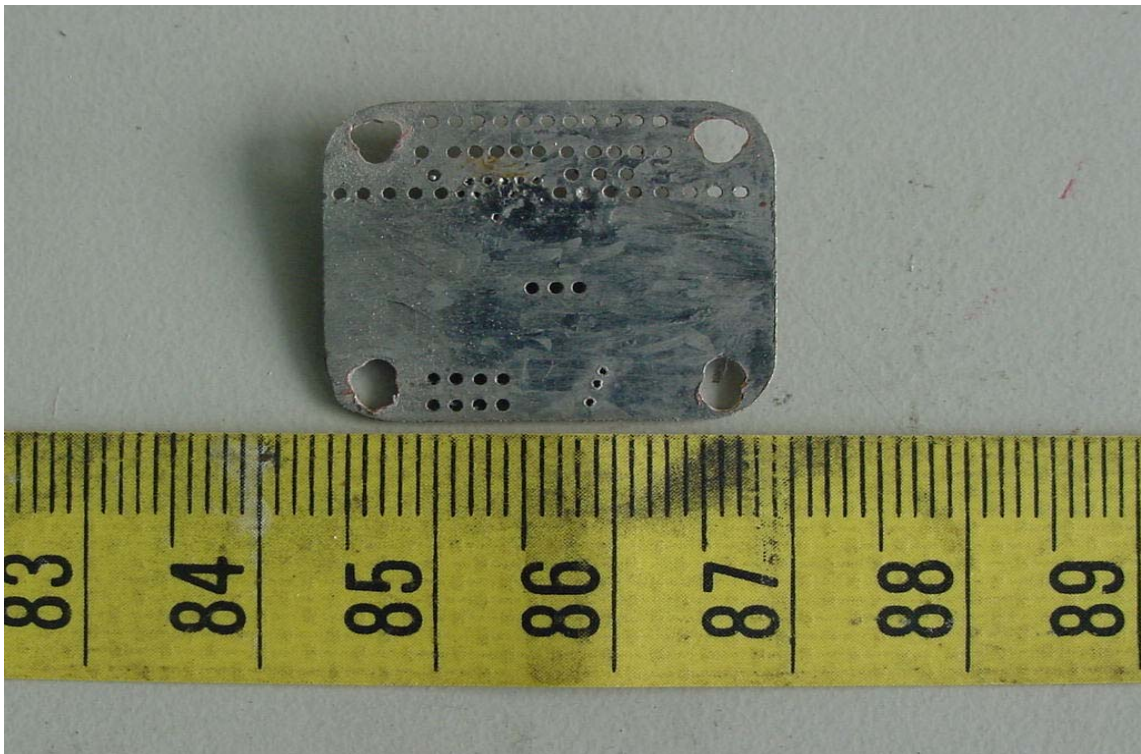
Solder View of CR Fitter's PCB
