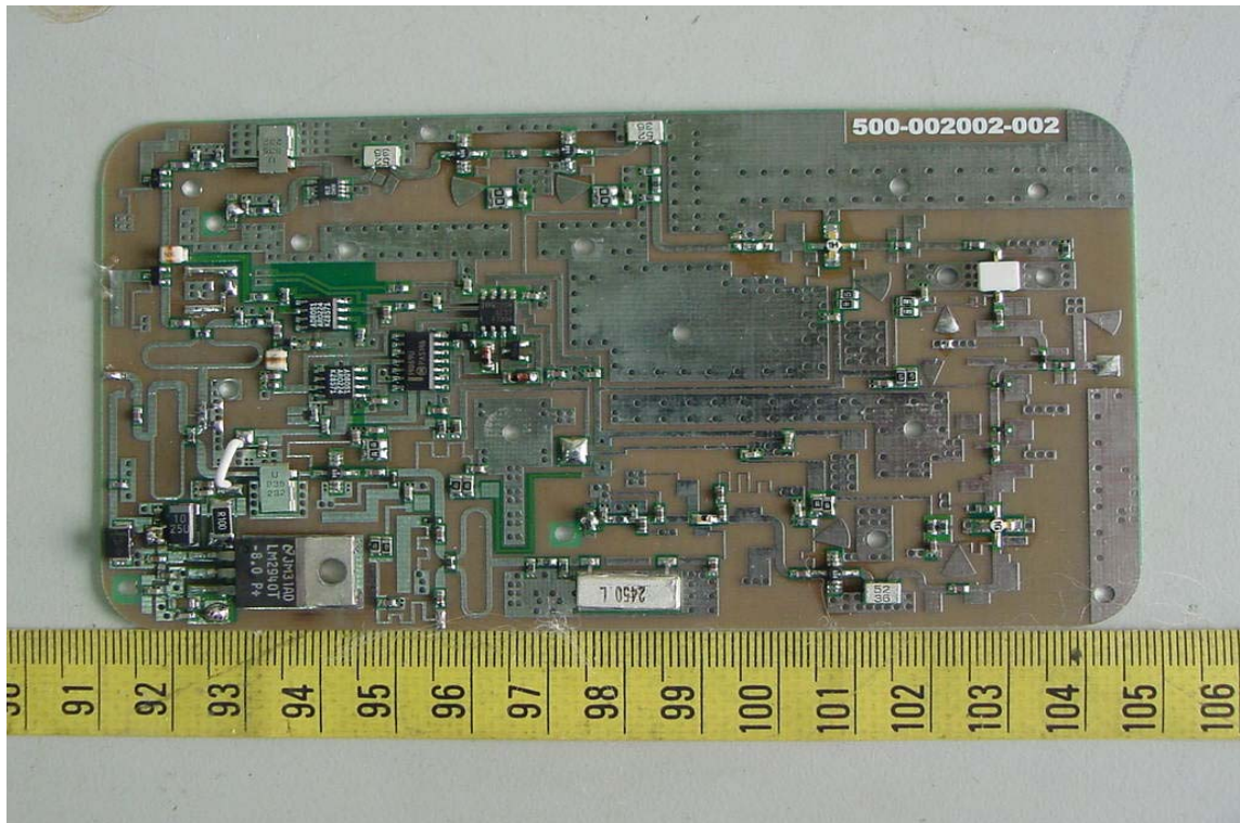
Component View of Converter's PCB
