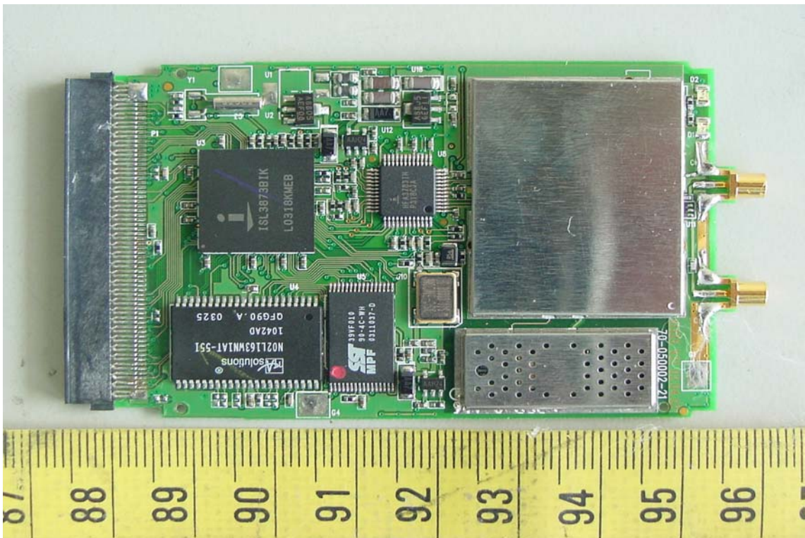
Component View of Wireless LAN Card PCB
