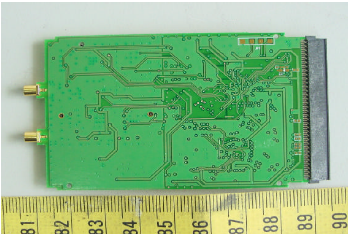
Solder View of Wireless LAN Card
