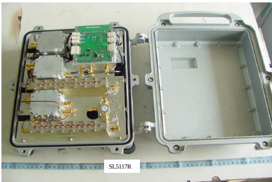
Internal View of ODU
