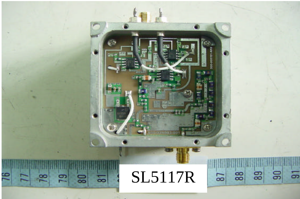
Solder View of ODU's PCB
