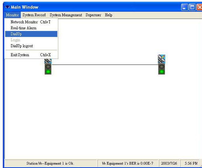
Figure 8-71 DialUp (1)
