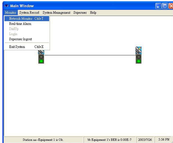
Figure 8-57: Network Monitor (1)
