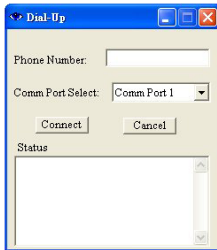
Figure 8-72 DialUp (2)
