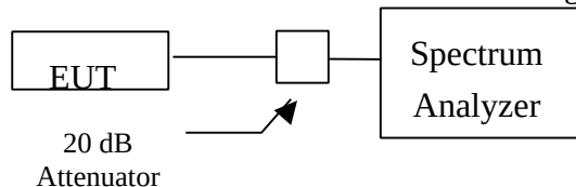
Figure 4: Emission bandwidth measurement configuration.
