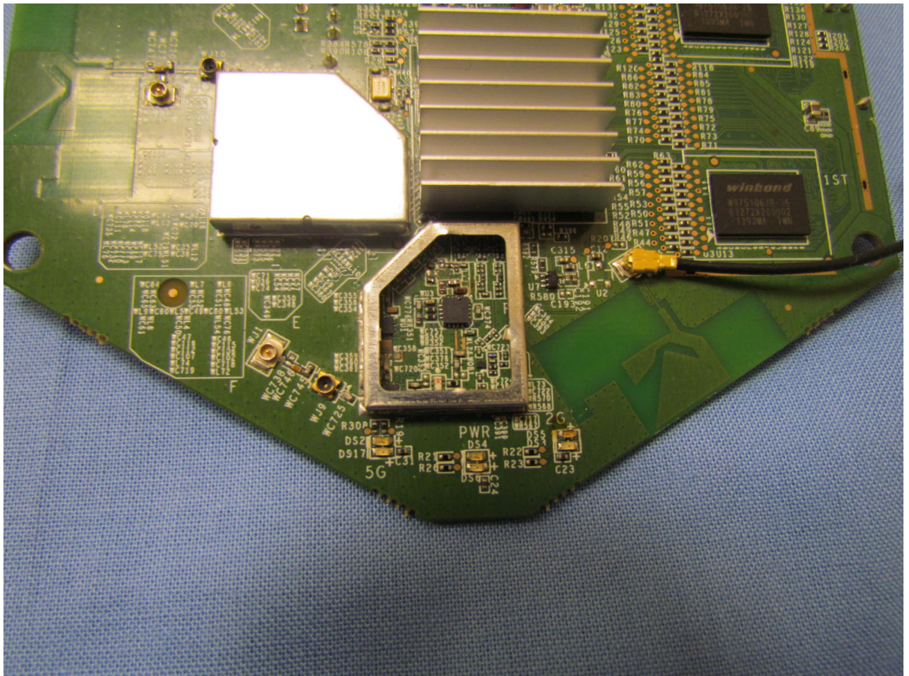
Main Assy back with shield 1 removed
