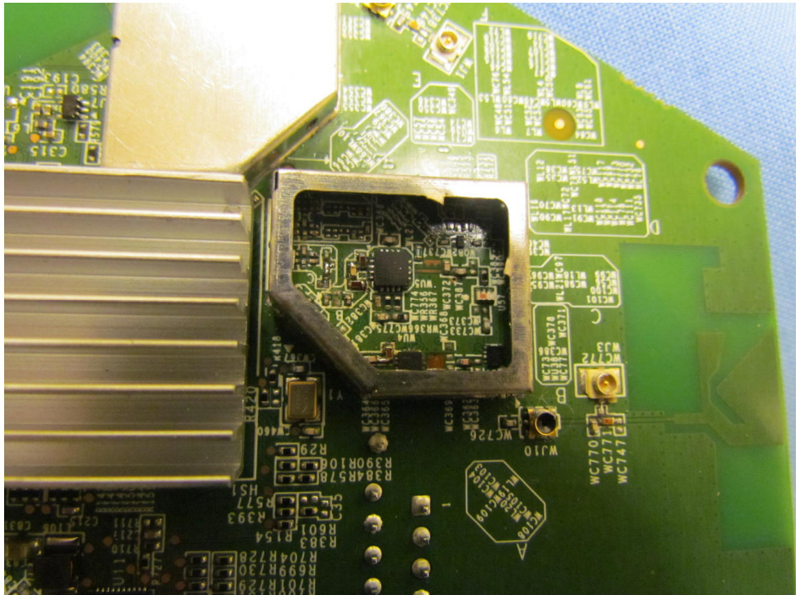
Main Assy back with shield 2 removed
