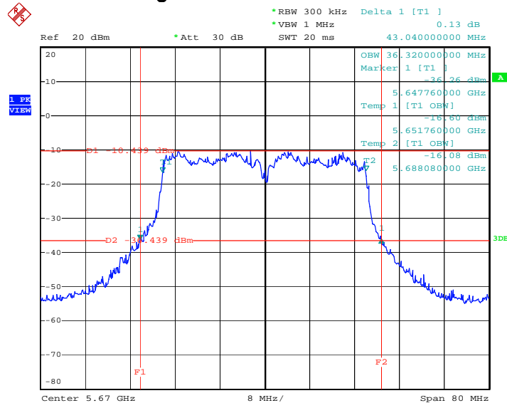
99% Occupied Bandwidth on Configuration Draft n MCS0 40MHz Ant. 4-1 + Ant. 4-3 / 5670 MHz
