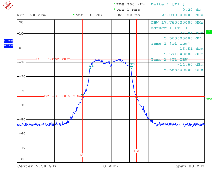
99% Occupied Bandwidth Plot on Configuration Draft n MCS0 20MHz Ant. 4-1 + Ant. 4-3 / 5580 MHz
