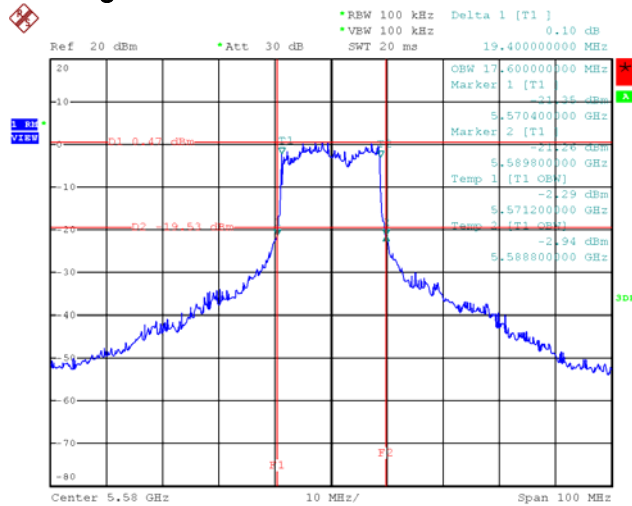
20dB Bandwidth Plot on Configuration Draft n MCS8 20MHz / 5580 MHz
