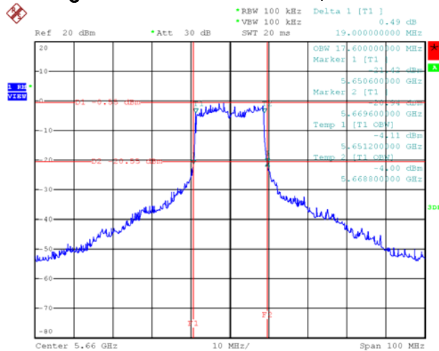
20dB Bandwidth Plot on Configuration Draft n MCS8 20MHz / 5660 MHz
