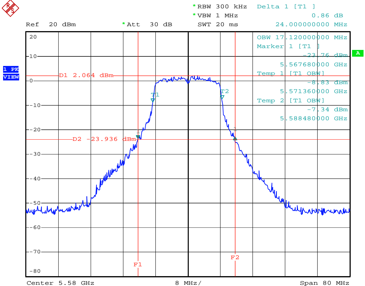
99% Occupied Bandwidth Plot on Configuration Draft n MCS0 20MHz Ant.A / 5580 MHz
