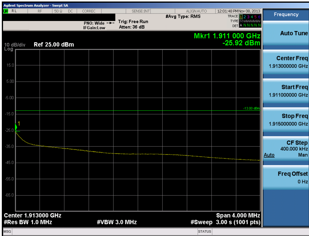
Plot 6-22. 4MHz Span Plot (PCS CDMA Mode – Ch. 1175)
