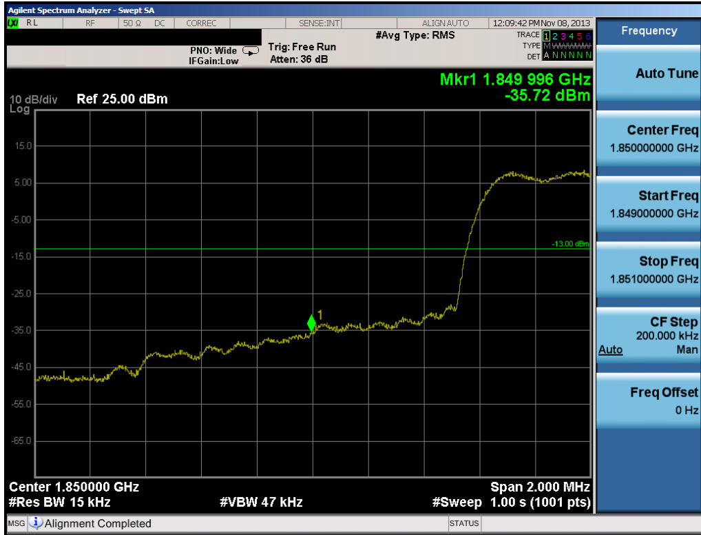
Plot 6-19. Band Edge Plot (PCS CDMA Mode – Ch. 25)
