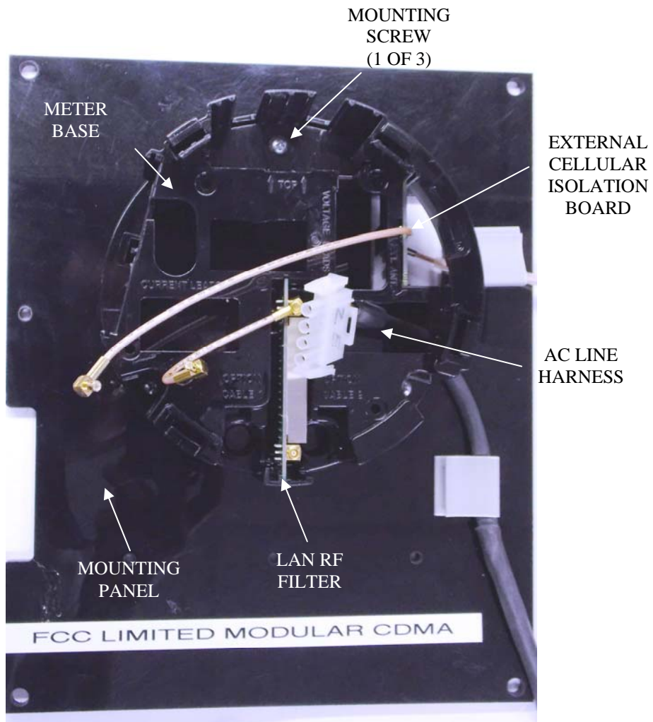
Modular EA_Gatekeeper base on plastic panel
