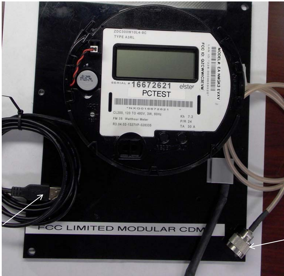
Modular EA_Gatekeeper complete module assembled to base
